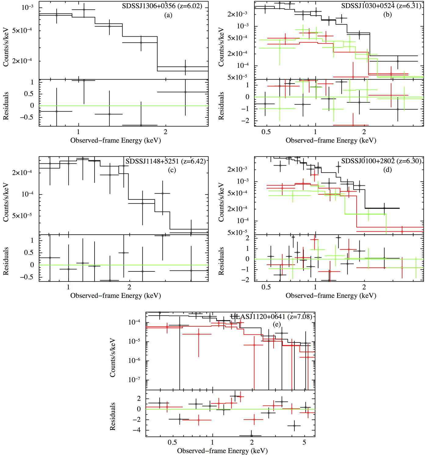
Fig. 4. Spectra of the five AGN with the best counting statistics ( 34 \leq \text{net counts} \leq 148 ). Spectra in panels a ) and c ) are extracted from Chandra , while spectra in panels b ), d ) and e ) are from XMM-Newton . The a ), b ) and d ) spectra are fit by a power-law model with Galactic and intrinsic absorption; the c ) and e ) spectra are fit by a simple power-law model plus Galactic absorption. The black, red, and green points and lines in the b ) and d ) panels correspond to pn, MOS1, and MOS2, respectively. The black and red points and lines in the e ) panel correspond to pn and combined MOS1 and MOS2, respectively. For the sake of clarity, we display the spectra using a minimum binning of 20, 15, 3, 3 and 20 counts for each bin for J0100+2802, J1030+0524, J1120+0641, J1148+5251 and J1306+0356, respectively.
