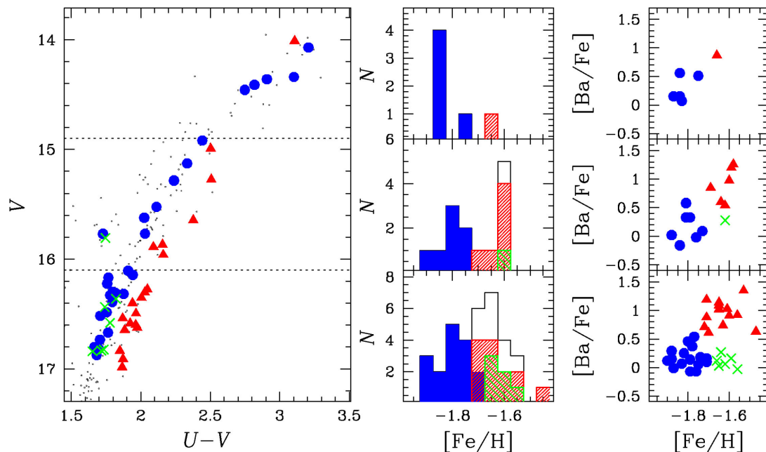
Figure 14. Left-hand panel: V-(U - V) CMD (left) of NGC 5286, corrected for differential reddening. Spectroscopic GIRAFFE targets are superimposed with s -rich/Fe-rich stars represented by red triangles, s -poor/Fe-poor stars by blue circles, and possible s -poor/Fe-rich stars by green crosses. Middle panels: histograms of [\text{Fe}/\text{H}] for GIRAFFE stars in the three different bins in V , represented on the V-(U - V) CMD. Right-hand panels: [\text{Ba}/\text{Fe}] versus [\text{Fe}/\text{H}] for stars in the three defined bins in V mag. Stars belonging to different Fe/ s -groups have been represented with different colours. The sources for the photometric data are given in Section 2.1.
