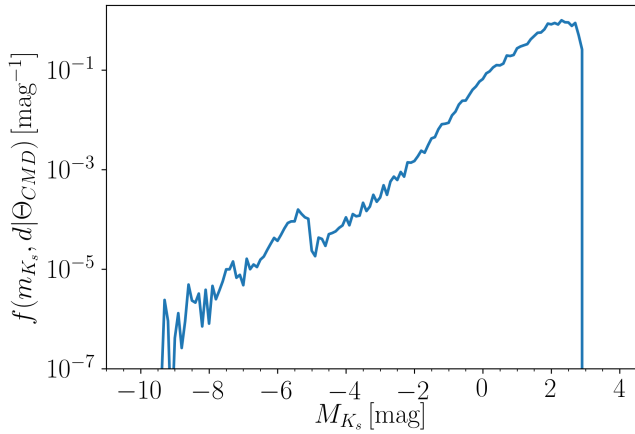
Fig. B.2. The effective luminosity function f(d, m_{K_s} | \Theta_{\text{CMD}}) used to determine our prior, normalised to unity.
