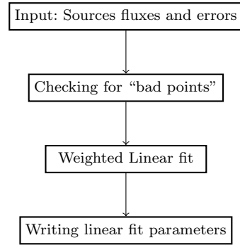
Figure 2. Spectral index extraction algorithm flowchart.
