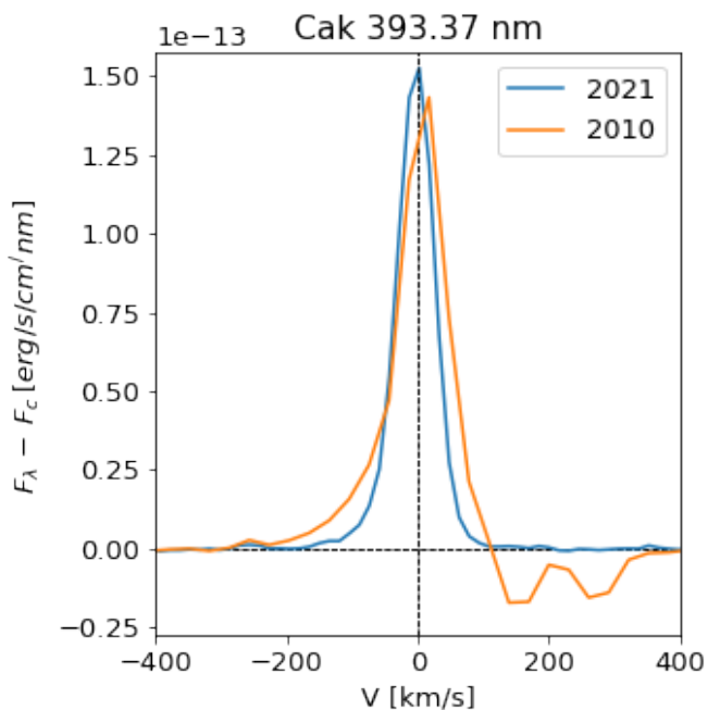
Fig. B.8. Profile of the CaK 393.37 nm line in the two X-Shooter observations.
