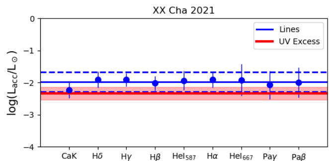
Fig. B.6. Comparison of the accretion luminosity derived from emission lines in the 2021 epoch with that derived from the UV excess. The mean accretion luminosity obtained from the lines is indicated with the solid blue line. The dashed lines indicates the error on the mean value. The accretion luminosity obtained from the UV excess is displayed with the red solid line and its error is shown via the shaded area.
