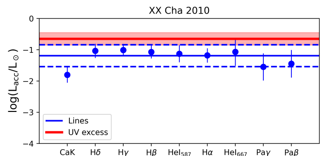
Fig. B.7. Comparison of the accretion luminosity derived from emission lines in the 2010 epoch with that derived from the UV excess. The mean accretion luminosity obtained from the lines is indicated with the solid blue line. The dashed lines indicates the error on the mean value. The accretion luminosity obtained from the UV excess is displayed with the red solid line and its error is shown via the shaded area.
