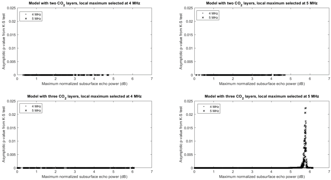
Fig. 11. Plots of the asymptotic p-values produced by the Kolmogorov-Smirnov test versus the maximum subsurface to surface power ratio of simulated echoes, for models with two- and three- \text{CO}_2 ice layers and for local maxima at 4 and 5 MHz. Each point represents the probability that model results and MARSIS measurements belong to the same continuous distribution. For each tested set of simulations, probabilities are computed both at 4 MHz (dots) and at 5 MHz (crosses).
