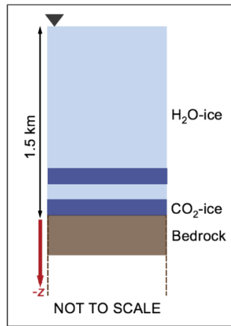
Fig. 9. Schematic stratigraphy used in numerical simulations. The model stratigraphy is here shown as a set of planar parallel layers of CO 2 ice (dark blue) and H 2 O ice (light blue), bounded by an upper half space representing the Martian atmosphere (as semi-infinite vacuum) and a lower half space representing the Martian bedrock (brown). Simulations are run for one, two or three lossless CO 2 ice layers, the lowermost of which is in direct contact with the bedrock, while the remaining ones are separated by layers of H 2 O ice of variable thickness. The topmost layer of H 2 O ice represents the bulk of the stratigraphy. Layer thicknesses of CO 2 ice and interlayer dusty water ice range from 0 to up to 100 m, with total deposit thickness = 1.5 km. The red arrow indicates the depth direction (-z). The inverted triangle on top of the sequence indicates the surface of the deposits. The sketch is drawn not to scale.
