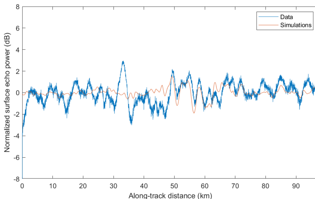
Fig. 6. Measured vs. simulated surface echo power for orbit 10737 at 4 MHz, both arbitrarily normalized to a 0 dB median power for ease of comparison.
