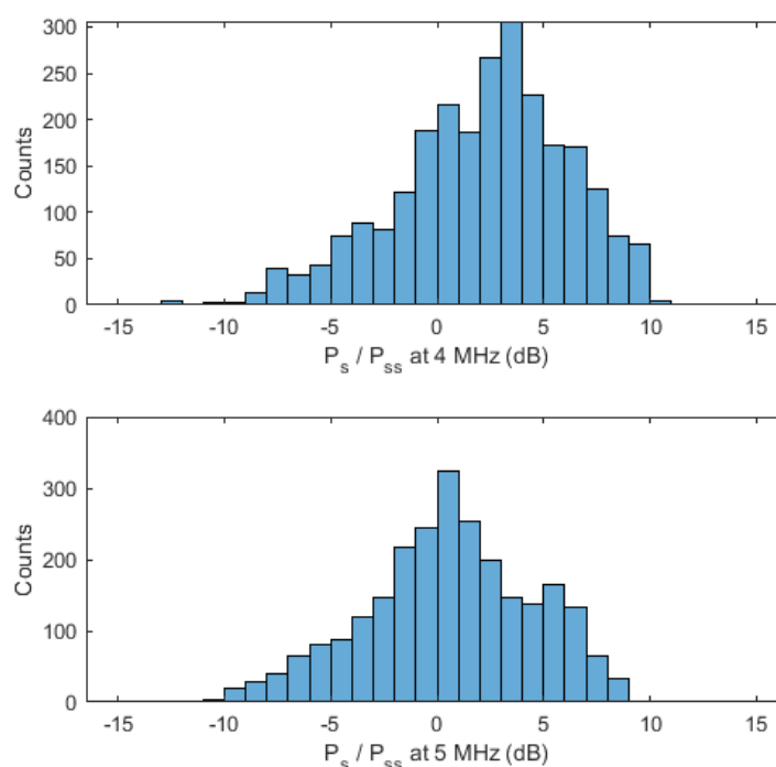
Fig. 7. Histograms of measured values of subsurface to surface echo power ratio over the bright reflector analysed in Orosei et al. (2018) at 4 MHz (top) and 5 MHz (bottom).
