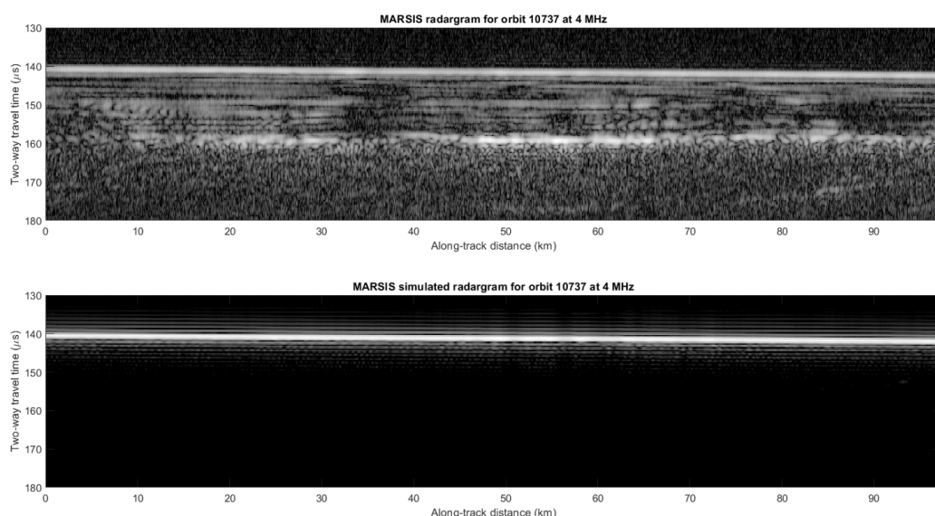
Fig. 5. Top: MARSIS radargram for orbit 10737 at 4 MHz, redrawn following Orosei et al. (2018), versus the corresponding simulation of surface scattering produced using the MOLA topographic dataset (bottom).
