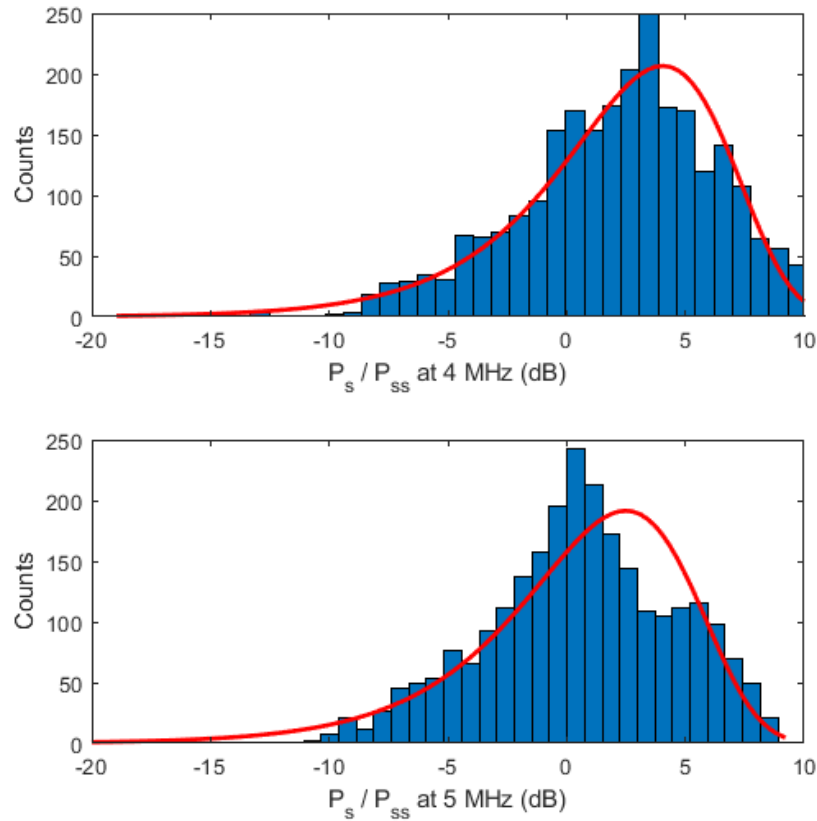
Fig. 8. Best-fit extreme value distributions plotted over the histograms shown in Figure 7.
