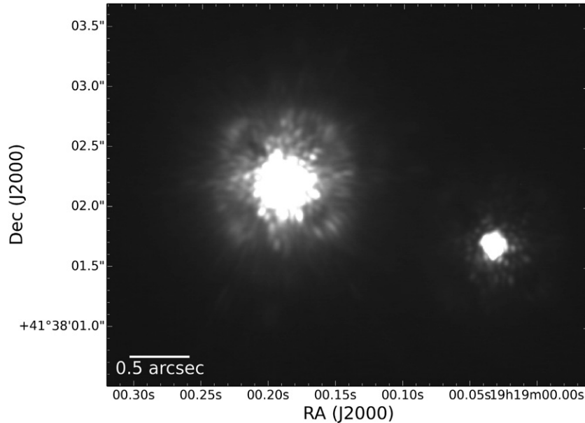
Figure 3. NIRC2 adaptive optics image of Kepler-444. The image was obtained using the K' filter ( 2.124 \mu\text{m} ) for a total of 378 s of integration time. Declination and right ascension coordinates (J2000.0) are given along the vertical and horizontal axes, respectively.
