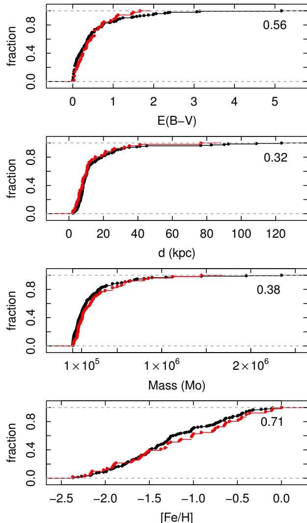
Fig. 1. Cumulative distributions of reddening, distance, stellar mass, and metallicity for GGCs in the top to bottom panels , respectively. Black curves represent the total sample (157 clusters) from the catalogue of Harris (1996, 2010 edition), and red curves are the sample from this work (51 clusters). The numbers in the panels are the p -values obtained by applying the Kolmogorov-Smirnov test to the black and red curves.
