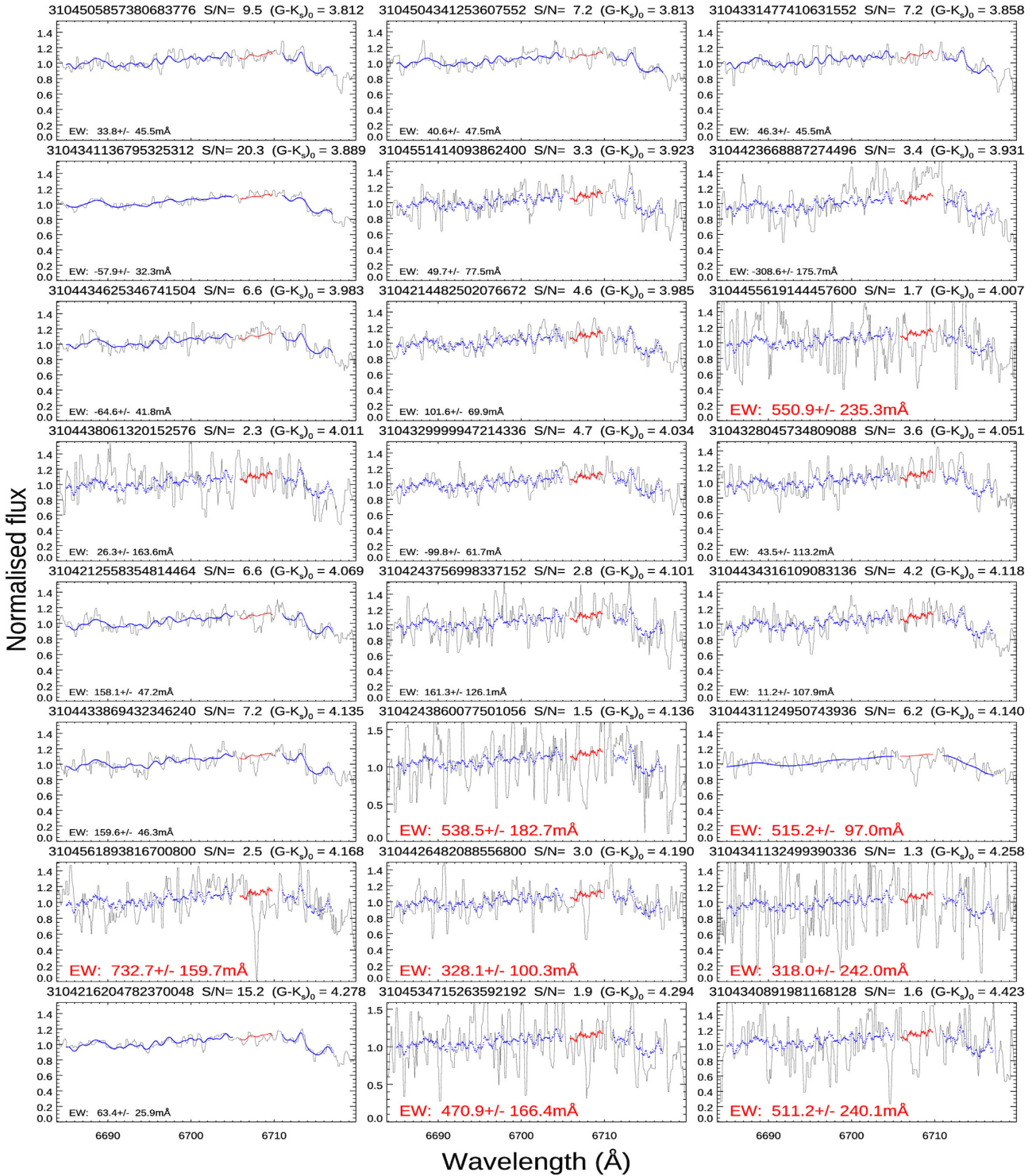
Figure 3. GES spectra for the 24 targets with (G - K_s)_0 > 3.8 . The normalized, reduced spectra from GESiDR5 are displayed in grey, where the data have been binned by 7 pixels. The best-matching spectral template (described in Section 3.2) is shown in the region encompassing the Li-feature at 6708 Å (in red) and in two regions either side of the feature (in blue). The title of each panel gives the Gaia DR2 source identifier, the S/N given in GESiDR5 and the (G - K_s)_0 colour. The EW(Li) values are provided in the bottom left of each panel, where targets defined as Li-rich are highlighted in larger red text.
