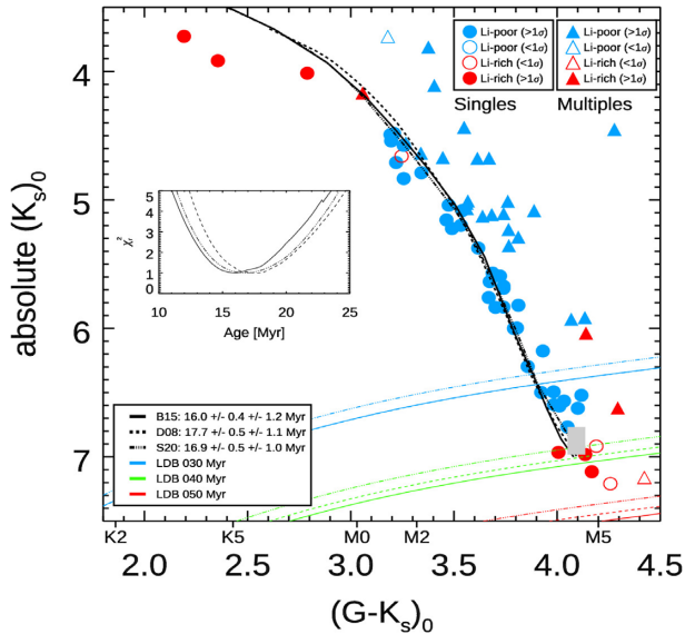
Figure 4. M_{K_s} versus (G - K_s)_0 for high probability cluster members. Red and blue symbols denote targets classed as Li-rich and Li-poor (in Section 4.1), where open and closed symbols denote whether the EW(Li) is within, or not within, one error bar of 300 mÅ. Circles and triangles represent the likely-single and likely-multiple stars (in Section 5), respectively. The grey box denotes the estimated position of the LDB. The blue, green, and red lines represent curves of constant luminosity at 99 per cent Li depletion from three standard models (see Section 4.2 for details) at 30, 40, and 50 Myr, respectively. The black curves are the best-fitting M_{K_s} versus (G - K_s)_0 isochrones to the likely single stars for the same models. The inset plot shows the reduced \chi^2_r as a function of isochrone age.
