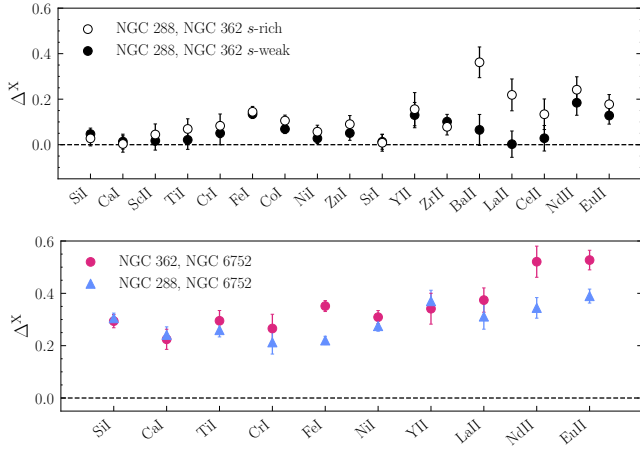
Figure 3. Comparison of the average abundance differences between NGC 288 and the two s -process groups in NGC 362 ( top ). The comparison with the s -weak group is shown using the filled circles, while the comparison between NGC 288 and the s -rich group is shown using open circles. Bottom , the differences between the two GCs in our study and the disc-like GC, NGC 6752 from Yong et al. (2013) (when considering all the stars in NGC 362, with the exception of the extremely s -process enhanced star NGC362-1441).
