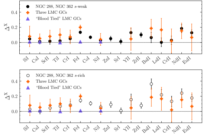
Figure 4. Comparison of the average abundance differences between NGC 288 and the two s -process groups in NGC 362 ( top : s -weak, bottom : s -rich) to the average differences between the three LMC GCs, NGC 1786, NGC 2210 and NGC 2257 (orange) and the binary (“blood tied”) LMC GCs, NGC 2136 and NGC 2137 (purple) from the studies of Mucciarelli et al. (2010) and Mucciarelli et al. (2012) respectively.
