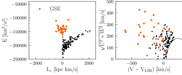
Figure 8. Selections of GSE stars from GALAH DR3 following several chemical, kinematic and dynamical cuts. The GSE selection is presented in orange, while a selection of in-situ stars is shown in black. The samples are shown in energy vs. z-angular momentum ( left ) and in the classical Toomre diagram ( right ). All orbital parameters are determined assuming a McMillan17 potential in galpy.
