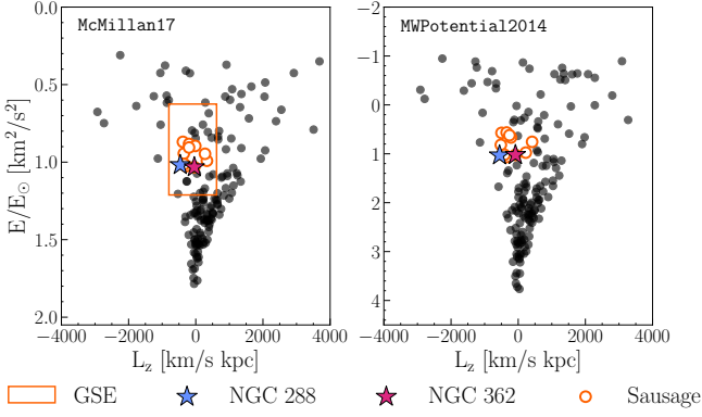
Figure 1. Energy ( E in \text{km}^2/\text{s}^2 ) scaled by solar energy vs. angular momentum ( L_z in \text{km/s kpc} ) for the majority of MW GCs calculated using the McMillan17 MW potential (as in the studies of Myeong et al. 2018; Massari et al. 2019), integrating for 2 Gyr (left). The extent of GSE in E vs. L_z as defined by Massari et al. (2019) is marked in orange, while the Sausage GCs identified by Myeong et al. (2018) are shown as the open orange circles. NGC 288 and NGC 362 are shown as the blue and pink stars respectively. The same information is shown for GCs integrated in the MWPotential2014 MW potential (right).
