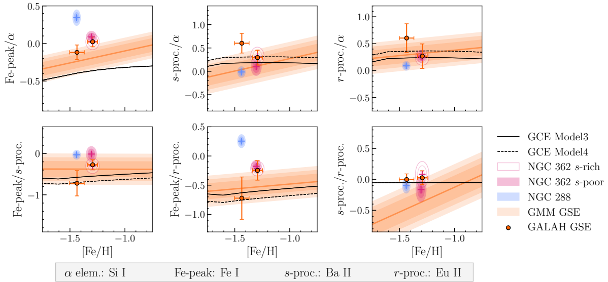
Figure 9. Predictions for the abundance ratios of four different nucleosynthetic channels (as characterised by the elements included in the key below the figure) from the two best-fit galactic chemical evolution models discussed in Sec. 4.2. Model parameters are given in Table 2 and discussed in Sec. 4.1. Average values for our two s -process groups in NGC 362, and a subset of GSE stars from GALAH are shown for each ratio. Trends for GSE predicted from the GMM of Myeong et al. (2022) are shown as the orange shaded regions marking the 1\sigma , 1.5\sigma and 2\sigma deviations from the predicted trends. Note that the GCE models are overlapping in the panel showing the prediction for the ratio of Fe-peak/ \alpha and s/r .
