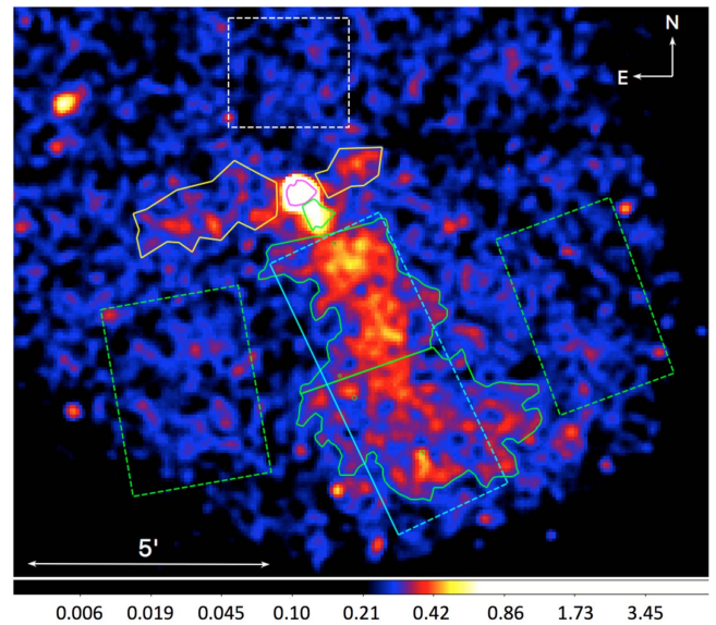
Figure 2. Merged 0.5–8 keV exposure-corrected image produced from all eight ACIS-I observations with point sources (detected by wavdetect ) removed. The image is binned by a factor of eight ( 3.9 pixel size), and smoothed with an r = 11.8 Gaussian kernel. The following spectral extraction regions are shown: the tail (green contour region; the line separates the “near” and “far” halves), and the “whiskers” (yellow polygons on either side of the CN). The two green dashed rectangles to the sides of the tail are the background regions used in the tail’s spectral fits. The cyan 2.5 \times 6.2 rectangular region (along the tail contour) is used to extract the tail brightness profile (see Figure 5). The CN (magenta polygon) and stem (green polygon) are also shown (same regions as in Figure 2), along with the background region (dashed white box) used in the pulsar, CN, stem, and whiskers spectral fits. The level for the green contour was chosen in such a way that it conforms to the tail morphology at the contrast shown. The color bar is in units of counts \text{arcsec}^{-2} .
