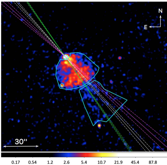
Figure 1. Merged exposure-corrected ACIS image (0.5–8.0 keV, smoothed with an r = 1.5 Gaussian kernel) with the following spectral extraction regions shown: pulsar/core ( r = 1.7 circle), compact nebula (CN) region (northern cyan polygon), and the mushroom “stem” region (southern cyan polygon). The magenta lines represent the direction of proper motion ( 48.4 \pm 2.1 east of north) as measured by Chatterjee et al. (2004), the white lines represent the direction of proper motion after the effects of solar motion and Galactic rotation have been removed ( 41.8 \pm 1.3 ; Hobbs et al. 2005), and the green lines represent the measured symmetry axis ( 34.7 \pm 0.6 ) of the CN (see below). The point source that appears near the southeastern trailing edge of the CN (shown by the crossed circular region) was excluded from the CN spectral analysis. The color bar is in units of counts \text{arcsec}^{-2} .
