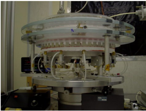
Fig. 8 The astatic equipment is used to support the shell during its fixation to the S3.
