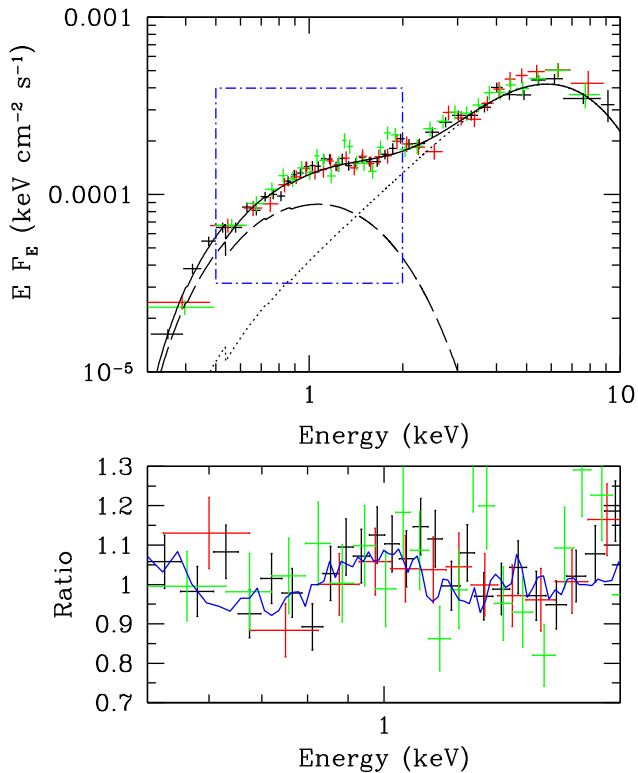
Figure 1. Upper panel: XMM–Newton spectral data points (PN: black, MOS1: red and MOS2: green) for P13 (re-binned for clarity). The best-fitting, unfolded model of \text{TBABS}^*(\text{DISKBB}+\text{NTHCOMP}) is shown as a solid line (see Table 1 for parameters and 1\sigma errors) with the \text{DISKBB} component shown as a dashed line and \text{NTHCOMP} as a dotted line. The blue, dot–dashed bounding box indicates the region of interest for the study of residuals to the model. Lower panel: 0.5–2 keV residuals to the best-fitting spectral model (same colour scheme as the upper panel). These cannot be adequately described by a constant at unity (null hypothesis probability <0.05 ) but resemble the residuals seen in other ULXs (Middleton et al. 2015b). For reference, the blue line indicates the smoothed residuals of the ULX NGC 1313 X-1 (Middleton et al. 2015b) which have since been unambiguously resolved into emission and absorption features associated with a relativistically outflowing wind (Pinto et al. 2016; Walton et al. 2016a).
