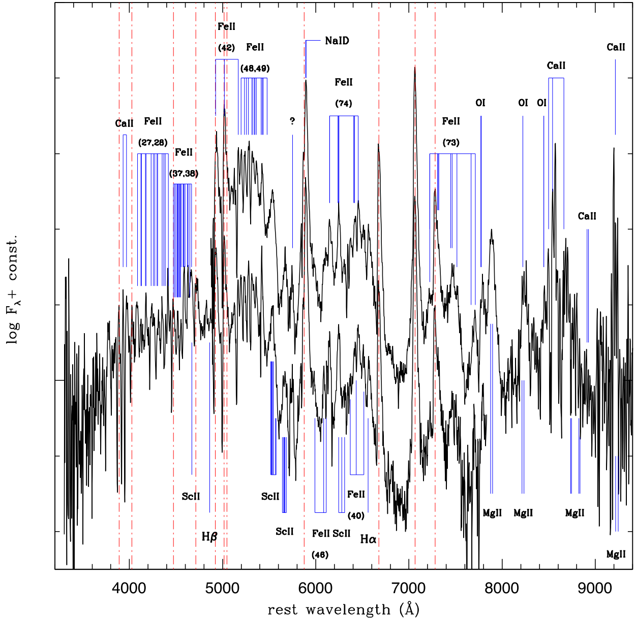
Figure 5. Identification of the most prominent lines in the late-time TNG spectra of SN 2014av. Dot-dashed vertical lines mark the rest wavelength positions of the strongest He I features.
