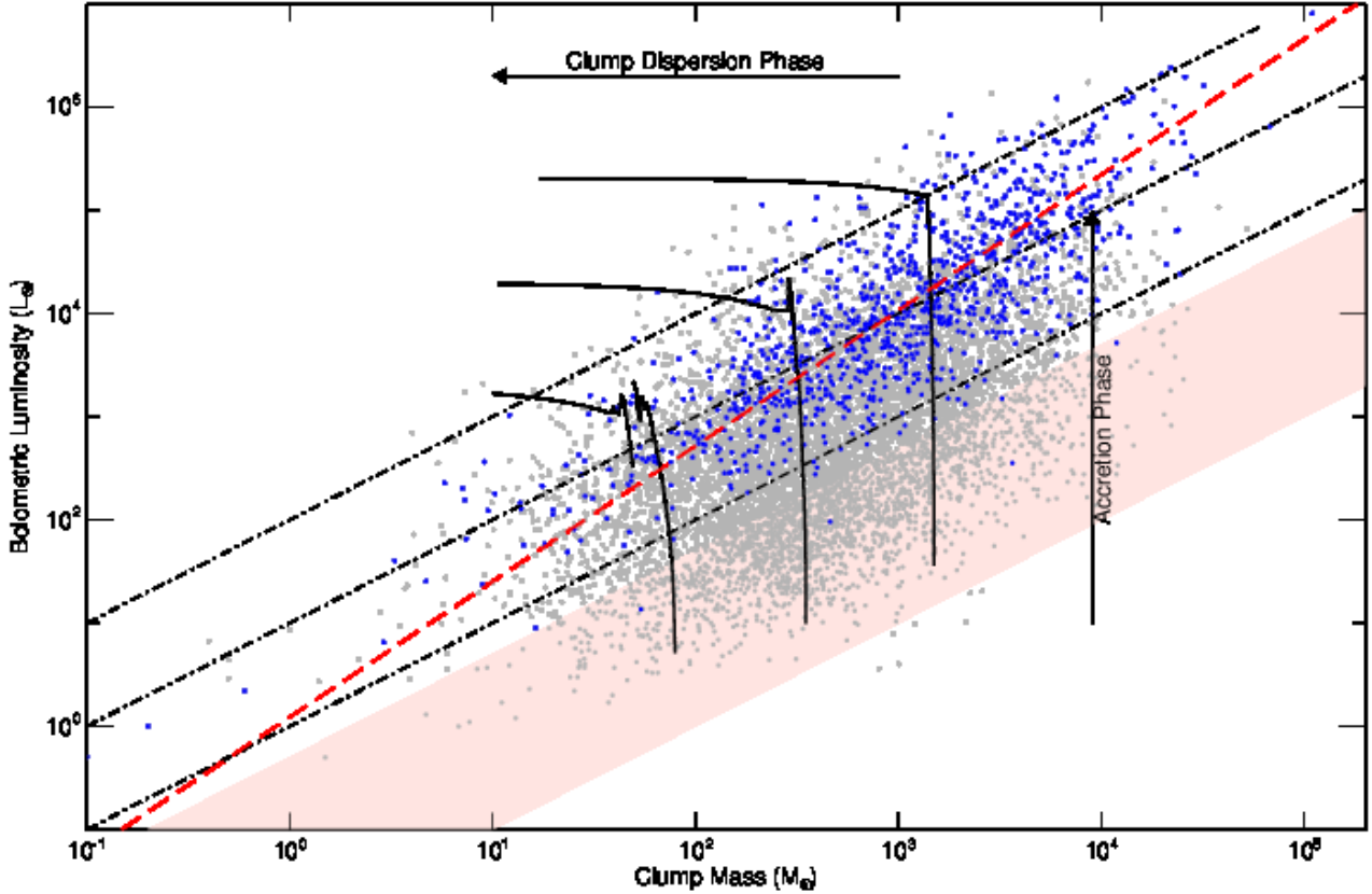
Figure 24. Clump mass-bolometric luminosity relationship for non-msf clumps (grey circles) and the MSF clumps (blue). The lower, middle and upper diagonal dash-dot lines indicate the L_{\text{bol}}/M_{\text{clump}} = 1, 10 and 100 L_{\odot}/M_{\odot} , respectively. The solid black curves, running respectively left to right, show the model evolutionary tracks calculated by Molinari et al. (2008) for stars with final masses of 6.5, 13.5 and 35 M_{\odot} , respectively. The light-red shaded area indicates the region of the parameter space we would expect to find quiescent clumps (temperatures between 10-15 K). The long-dashed diagonal red line shows the results of a log-log, outlier-resistant, linear fit to the MSF clumps; this has a slope of 1.314 \pm 0.0189 and an intercept of 0.087 \pm 0.056 .
