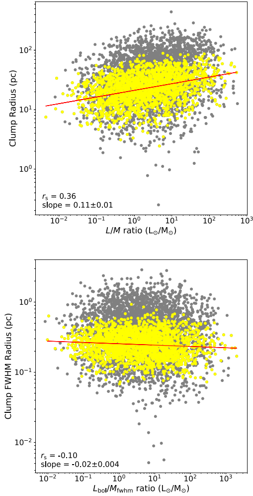
Figure 9. The upper panel presents the clump radius versus clump L/M ratio for previously calculated values of radius, luminosity, and mass within the ATLASGAL survey. The lower panel presents clump FWHM radius against clump L_{\text{bol}}/M_{\text{fwhm}} ratio, for the newly derived clump sizes (see Section 4.2). Both plots present the entire ATLASGAL sample and a distance limited sample (2–4 kpc) in grey and yellow respectively. The results from a Spearman’s rank correlation coefficient test for the distance limited samples (2–4 kpc) is shown in the lower left of each panel, the p -value for both distributions is below our significance threshold.
