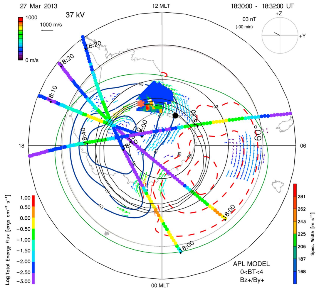
Figure 7. The South Pole Doppler spectral width measurements overlotted on the convection map of 18:30 UT.
