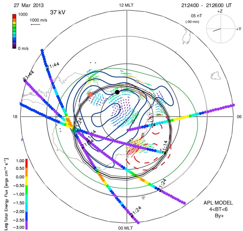
Figure 6. Global ionospheric convection maps for 2 min intervals starting at (a) 18:30 UT and (b) 21:24 UT.
