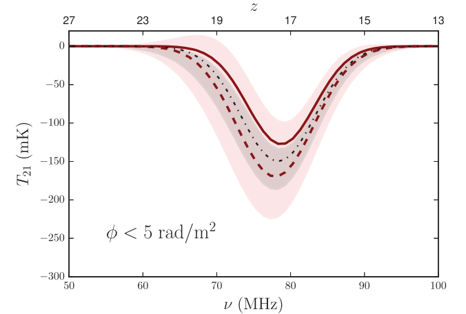
Figure 9. The black dotted–dashed line is the Gaussian fiducial input signal in the LF band. We show here reconstructed T_{21,\text{G}} signal considering the ‘low \phi ’ (i.e. \phi < 5 \text{ rad m}^{-2} ) case with signal magnitude reduced to the 10 per cent of the reference simulation – see text for details. The red (grey) shaded area is the 1\sigma region around the mean for the xx ( yy ) polarization. The solid (dashed) red line shows one of the reconstructed T_{21,\text{G}} signal for the xx ( yy ) polarization.
