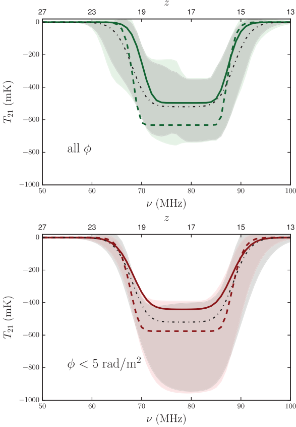
Figure 7. The black dotted–dashed line in both panels is the input signal: the best-fitting flattened Gaussian from Bowman et al. (2018a). Top panel: reconstructed T_{21,\text{FG}} signal in the case of the ‘all \phi ’ simulations, in the LF, from the Bayesian analysis described in the text. The solid (dashed) green line shows one of the reconstructed T_{21,\text{FG}} signals for the xx ( yy ) polarization. The green (grey) shaded area is the 1\sigma region around the mean for the xx ( yy ) polarization (see text for details). Bottom panel: same as top panel but for the ‘low \phi ’ (i.e. \phi < 5 \text{ rad m}^{-2} ) simulations. The red (grey) shaded area is the 1\sigma region around the mean for the xx ( yy ) polarization, and the solid (dashed) red line shows one of the reconstructed signal for both xx ( yy ) case.
