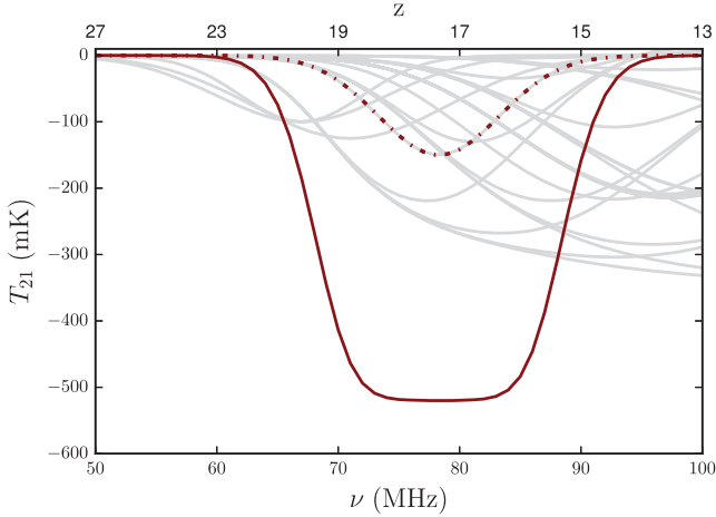
Figure 2. Our fiducial Gaussian input model (dot-dashed red line) and the flattened Gaussian model best fit of the EDGES data (Bowman et al. 2018a, solid red line), compared with the global signal profiles obtained with SIMFAST21 (Santos et al. 2010) varying the physical input parameters (solid grey lines).
