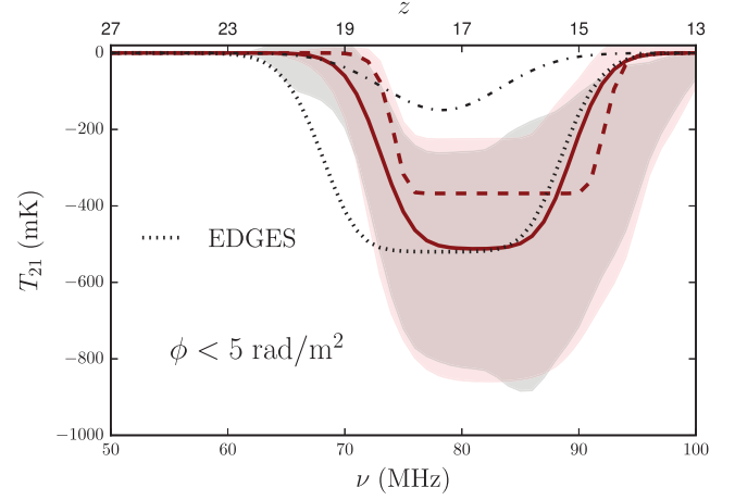
Figure 8. Reconstructed T_{21,\text{FG}} signal. Note that the input signal is the fiducial Gaussian model (black dotted–dashed). The solid (dashed) red line shows one of the reconstructed T_{21,\text{FG}} signals for the xx ( yy ) polarization. The red (grey) shaded area is the 1\sigma region around the mean for the xx ( yy ) polarization (see text for details). For comparison we also show the EDGES best fit (dotted line).
