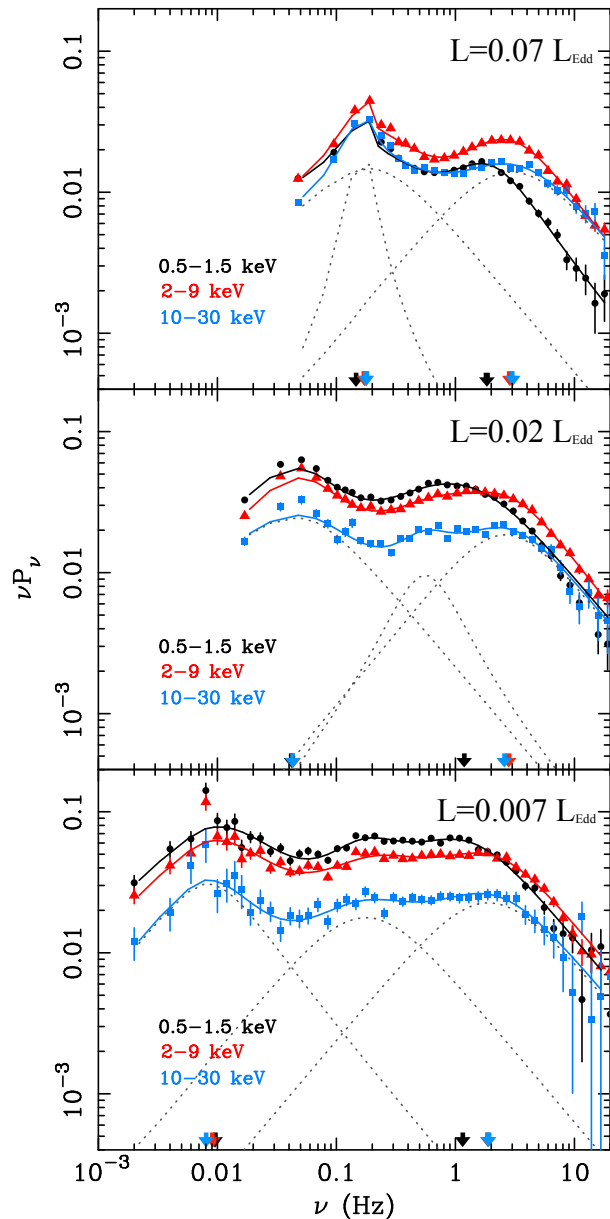
Figure 2. The PSDs of GX 339-4 in the three energy bands 0.5–1.5 keV ( soft ), 2–9 keV ( hard ), and 10–30 keV ( very hard ), for each observation at different luminosity. The arrows mark the best-fit peak frequency of the low-frequency ( \nu_l ) and the high-frequency ( \nu_h ) Lorentzians for each energy band.
