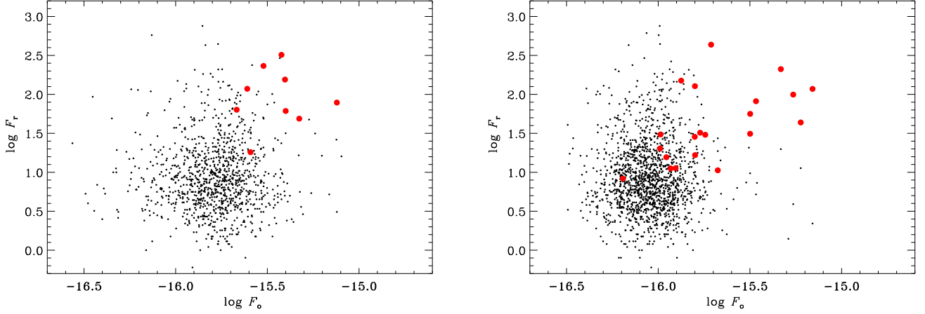
Fig. 14. Left panel: the flux density of the FIRST central component, F_r , versus dereddened flux density within the SDSS fiber at 3900 \text{ \AA} , F_0 , for the sources with 0.05 < z \leq 0.1 . The candidate BL Lacs are plotted with red circles. Right panel: same as in the left panel, but for 0.1 < z \leq 0.15 .
