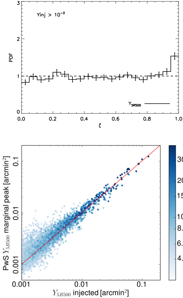
Fig. 13. Top: results of the posterior validation for Y_{5R500} . The histogram of the posterior probability, \zeta , bounded by the true Y_{5R500} parameter, is almost uniformly distributed, except for a small excess in the tails of the posteriors, at \zeta > 0.95 . The histogram has been normalised by the expected counts in each \zeta bin. Bottom: comparison of recovered peak Y_{5R500} to the injected Y_{5R500} . The estimates are unbiased, though asymmetrically scattered, with a scatter that decreases as S/N increases.
