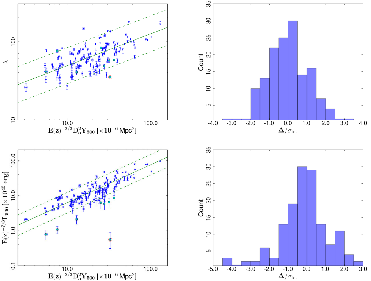
Fig. 28. Properties in the Y_{500} – \lambda (top panels) and Y_{500} – L_{500} (bottom panels) planes for the Planck -redMaPPer sample at z < 0.2 . Under-luminous candidates are denoted with cyan circles in the scatter plots to the left, which also show the best fit relation and the dispersion \pm 2\sigma_{\text{tot}} . The circled red point is a cluster with contaminated Y signal. The right plots show the histograms of orthogonal deviation \Delta_{\perp} for each relation.
