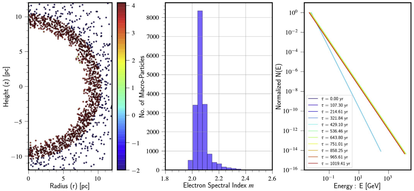
Figure 11. Left panel: particle distribution at time \tau = 1008 yr for the SN 1006 supernova remnant case. The colors represent the compression ratio due to shock while the negative values represent initial particles in the domain that have not interacted with the shock. Middle panel: histogram showing the electron spectral index m for all the particles that have been shocked. Right panel: evolution of spectral energy distribution for a single representative macro-particle.
