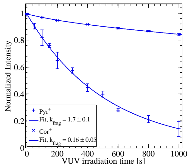
Fig. 5. Normalized intensity of Pyr + and Cor + as a function of the VUV irradiation time. The fitting curves and the extracted fragmentation rates (see method in Sect. 2.4) are displayed for each species with k_{\text{frag}} in 10^{-3} \text{ s}^{-1} .
