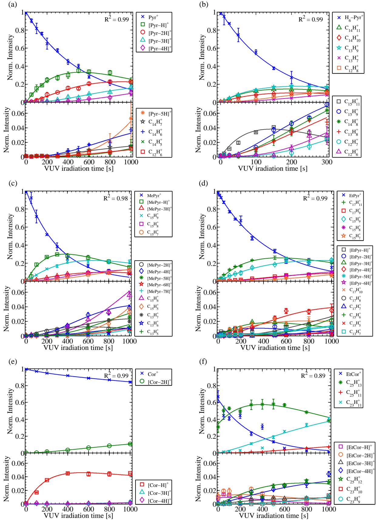
Fig. B.1. Kinetic curves of the studied PAH cations and their fragments: (a) \text{Pyr}^+ , (b) \text{H}_6\text{-Pyr}^+ , (c) \text{MePyr}^+ , (d) \text{EtPyr}^+ , (e) \text{Cor}^+ , (f) \text{EtCor}^+ ( \text{MeCor}^+ is shown in Fig. 4a). For each figure, the top panel shows the main channels while the bottom panel is a zoom on the minor channels. The solid curves correspond to the fitting functions that were derived with the procedure described in Sect. 2.4. The derived photofragmentation maps are shown in Figs. 6, 8, and 9.
