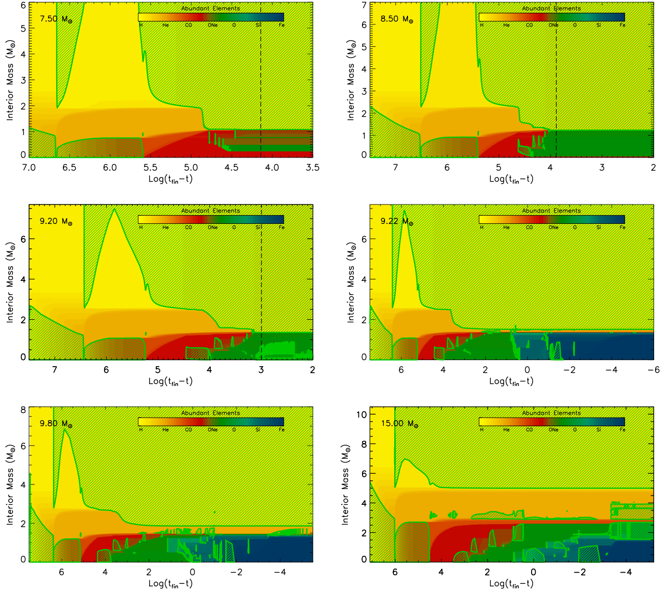
Figure 1. Convective (green shaded areas) and chemical (color codes reported in the color bar) internal history of selected models from the main-sequence phase up to an advanced stage of the TP-SAGB phase (top and middle left panels) or the onset of the iron core collapse prior to the CCSN explosion (middle right and bottom panels). The dashed line in the top and middle left panels marks the onset of the TP phase. The x-axis reports the logarithm of the time until the end of the evolution ( t_{\text{fin}} - t ) in units of years.
