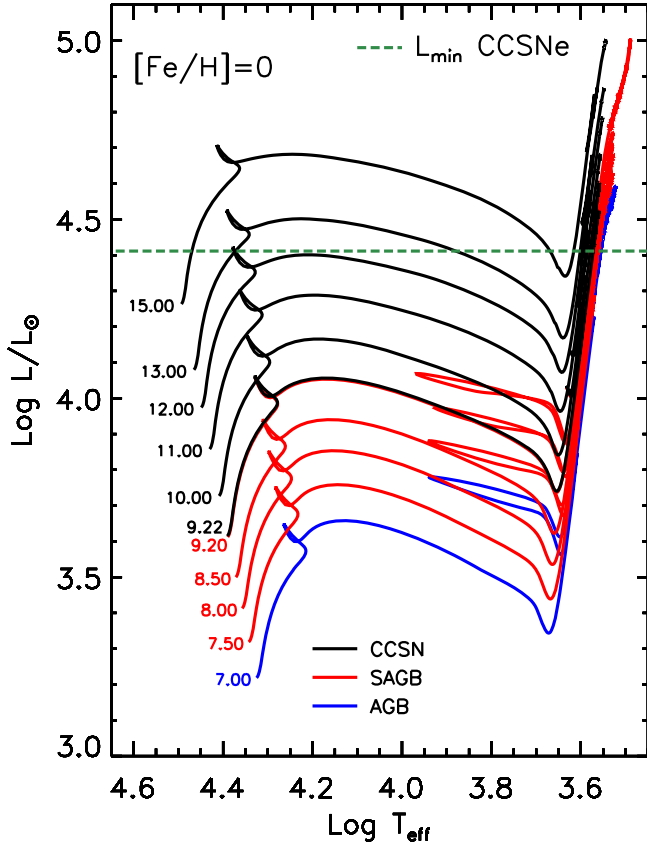
Figure 2. Evolutionary path in the H-R diagram of selected models. The blue line refers to the AGB star, i.e., the one that develops a degenerate CO core, does not ignite C burning, and enters the TP phase. The red lines refer to SAGB stars, i.e., those that ignite C burning and then do not ignite Ne burning; these stars develop a degenerate ONeMg core and enter the TP phase. The black lines refer to those stars that ignite Ne burning and eventually explode as CCSNe. The horizontal green dashed line marks the final luminosity of the lowest mass that explodes as CCSNe, i.e., the expected minimum luminosity of CCSNe (Smartt 2015).
