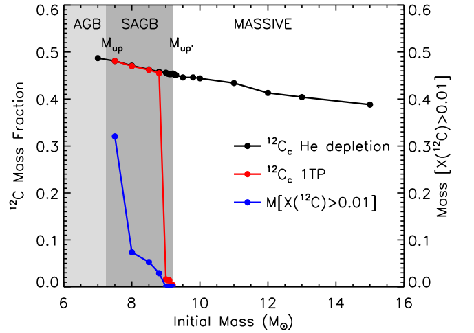
Figure 5. Central ^{12}\text{C} mass fraction at core He depletion (black line and dots) and at first thermal pulse (red line and dots). The blue line refers to the mass of the central zone where the ^{12}\text{C} mass fraction is larger than 0.01. The figure shows that the models with initial mass between 7.5 and 8.8 M_{\odot} form a hybrid degenerate CO core.
