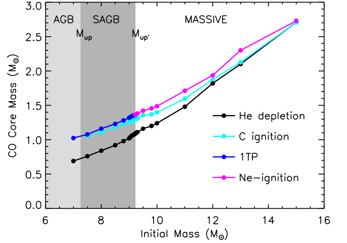
Figure 4. CO core mass at various evolutionary stages (see legend).
