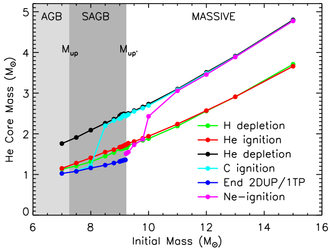
Figure 3. He core mass at various evolutionary stages (see legend).
