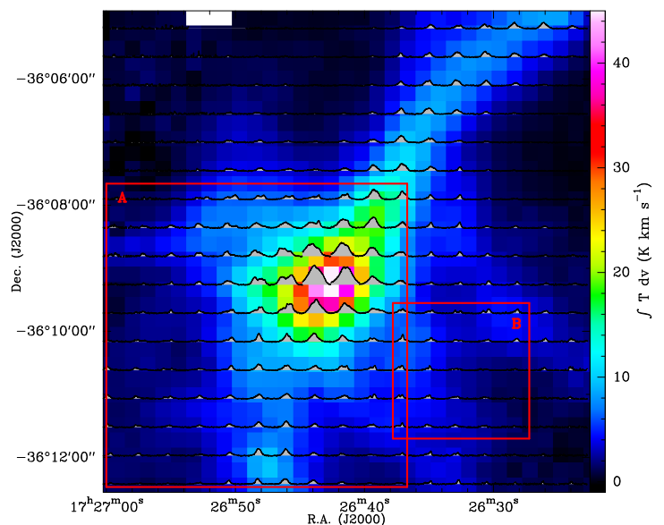
Fig. 6. Map of the \text{C}^{18}\text{O} (2–1) transition overlaid on the integrated emission of the same line in the velocity range [-6, -1]\text{ km s}^{-1} . The red boxes indicate the regions shown in Fig. 7.
