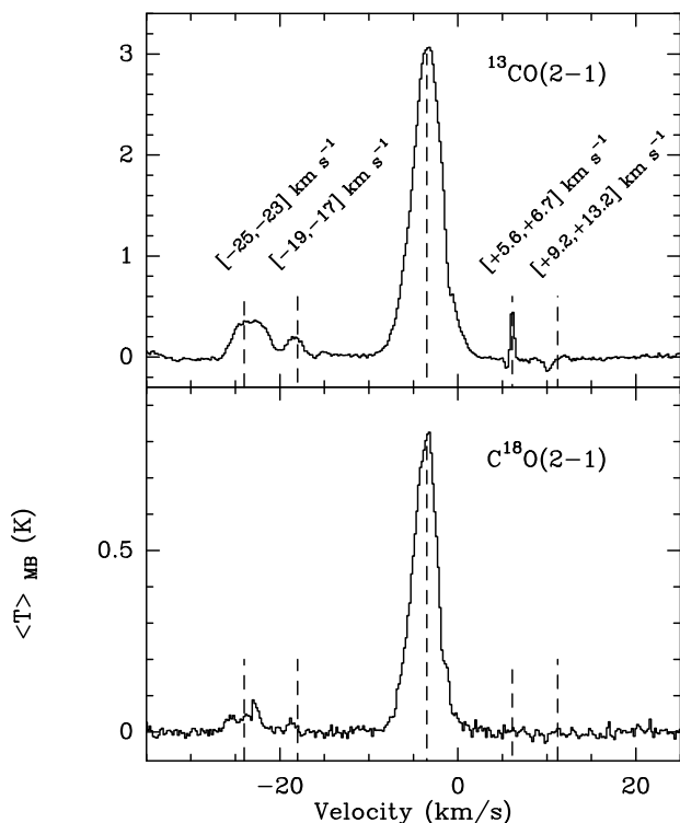
Fig. 5. Averaged ^{13}\text{CO} (2–1) (top) and \text{C}^{18}\text{O} (2–1) (bottom) spectra over the full extent of the APEX map. The dashed lines indicate v_{\text{LSR}} of -18\text{ km s}^{-1} , -24\text{ km s}^{-1} , -3.5\text{ km s}^{-1} , +6\text{ km s}^{-1} , +11\text{ km s}^{-1} . The velocity ranges used to obtain the integrated intensity maps shown in Fig. A.4 are also shown.
