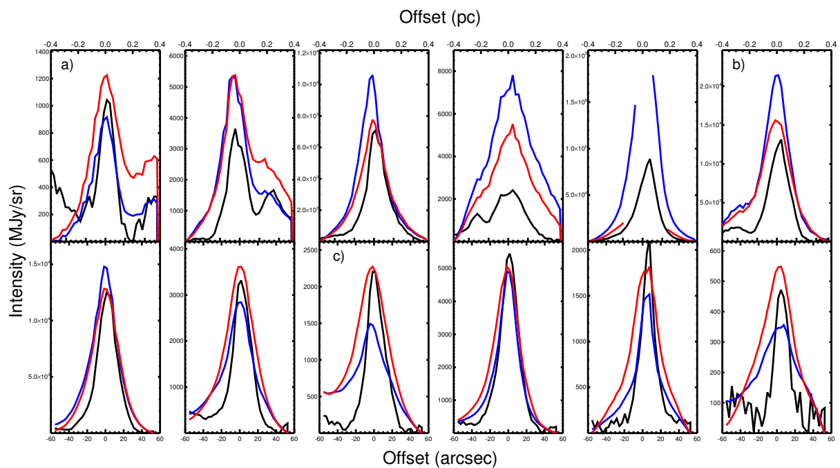
Fig. A.2. Average radial profile of G351 estimated from the SABOCA emission at 350\ \mu\text{m} emission (solid black line), Hi-GAL- 250\ \mu\text{m} (red), and Hi-GAL- 160\ \mu\text{m} data (blue). The panels show the 12 regions of Fig. 4 ordered from top left to bottom right.
