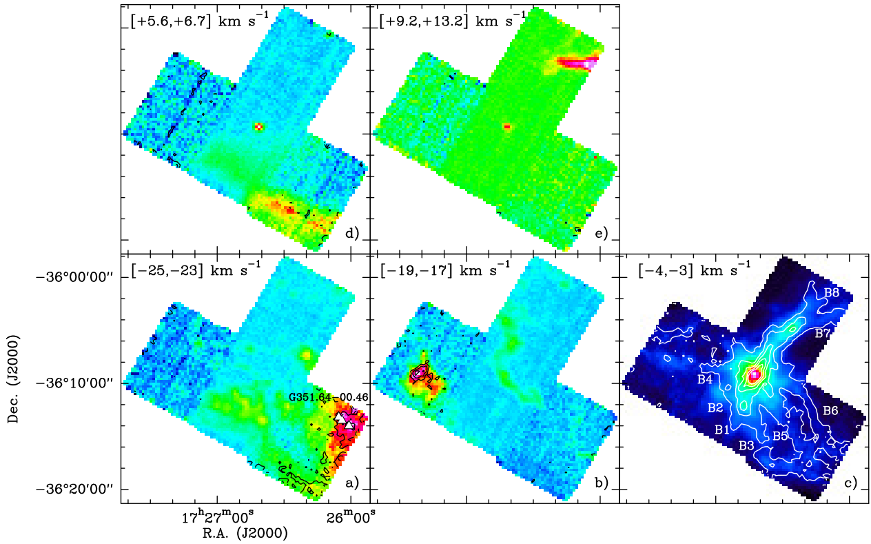
Fig. A.4. Integrated emission of the ^{13}\text{CO} (2–1) line over five different velocity ranges (see Fig. 5) is shown in colour scale. The point-like emission seen towards Clump-1 in the [+5.6, +6.7] \text{ km s}^{-1} and [+9.2, +13.2] \text{ km s}^{-1} velocity ranges is due to high-velocity emission associated with molecular outflows (see Leurini et al. 2009). Black contours show the corresponding integrated \text{C}^{18}\text{O} (2–1) emission from 30% of its peak emission in steps of 30%. The white contours in the bottom right panel show the integrated \text{C}^{18}\text{O} (2–1) emission in the range -3.5 \pm 0.5 \text{ km s}^{-1} from 5% to 45% of the corresponding peak emission in steps of 10%. The B1–B8 labels are as in Fig. 1.
