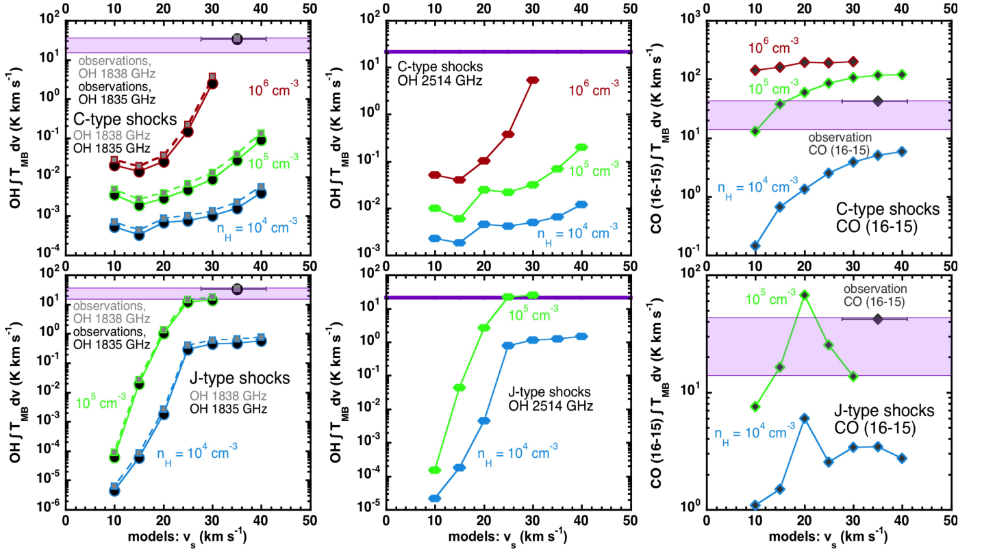
Fig. 4. Comparisons of the integrated intensities (Main beam temperature units) of all observed lines with the predictions of our grid of C-type ( Upper panels ) and J-type ( Lower panels ) models. In all panels, the abscissa is the shock velocity. In all panels, the colour symbols are the model predictions, where the red, blue, and green filled circles correspond to the pre-shock densities indicated in each panel. Finally, in all panels, the grey and black points are the observations integrated over the whole redshifted shock component (scenario 1, section 5.1), while the pink area corresponds to the range of values that correspond to the LV and HV values, see Table 5, in turn corresponding to scenario 2, section 5.2. In the central panels, the purple line is the observed intensity integrated between -90 and -20 \text{km s}^{-1} . Left-hand side panels: OH at \sim 1835 GHz and \sim 1838 GHz. The computed 1835 GHz and 1838 GHz intensities are connected by continuous and broken curves, respectively. The observed intensities are indicated by black (1835 GHz) and grey (1838 GHz) points with horizontal bars, reflecting the uncertainty on the shock velocity; the uncertainty on the intensity are of the order of the points sizes (see text). Central panels: OH at \sim 2514 GHz. Right-hand side panels: CO (16–15).
