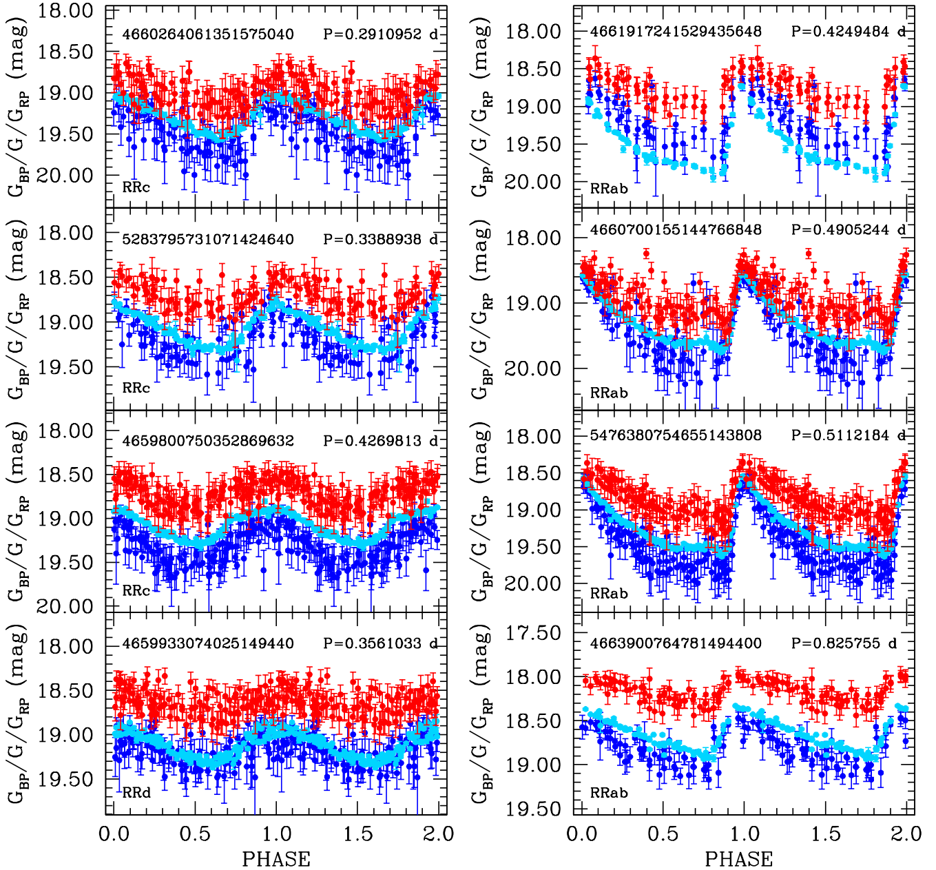
Fig. 13. G (cyan), G_{BP} (blue), and G_{RP} (red) light curves of RR Lyrae stars of different pulsation mode in the LMC and SMC, released in Gaia DR2. The multi-band time-series data are folded according to the period and epoch of maximum light derived by the SOS Cep&RRL pipeline. Although the errors are larger than in the G band, the colour light curves are well defined. The G_{BP} light curve of the RR Lyrae star in the top right panel is brighter and has a lower amplitude than the G -band curve, likely because the star is blended with a companion that contaminates the G_{BP} photometry (see Sect. 4.1 for details).
