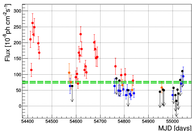
Fig. 13: Light curve of 3C454.3 in the energy range 100 MeV – 10 GeV, with a four-day resolution. The black downward arrows represent 2\sigma upper limits. The blue, orange, and red circles refer to a \sqrt{TS} value \geq 3 , \geq 4 , and \geq 5 , respectively. The green dashed lines indicate the average flux plus/minus the error from Table 10
