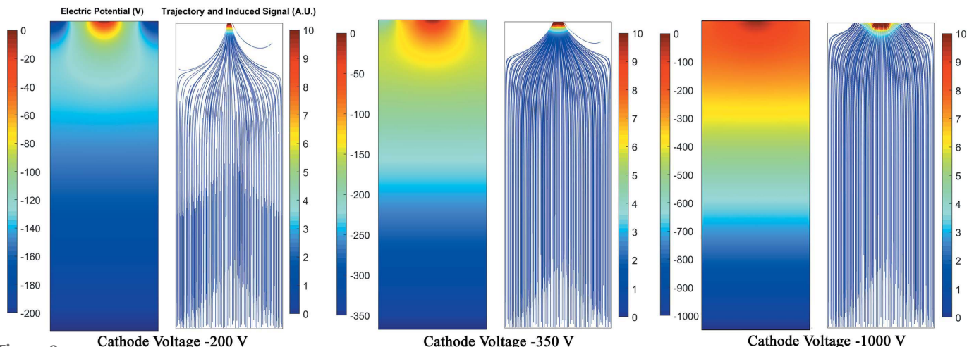
Figure 8 Calculated electric potential and simulated electron induced current at different cathode voltages (adjacent drift strips: -100 \text{ V} ; central drift strips: -200 \text{ V} ). The results clearly show that the induced current on the collecting anode strip is enhanced at -350 \text{ V} .
