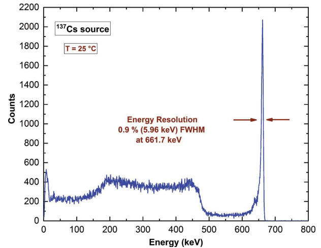
Figure 15 Measured uncollimated 137 Cs energy spectrum from a collecting anode strip after spectral correction. The energy spectrum is obtained with the collecting anode strip events in temporal coincidence with all pulses from drift and cathode strips. The correction was only applied to the anode strip pulses in temporal coincidence with the induced-charge pulses with negative saturation levels.
