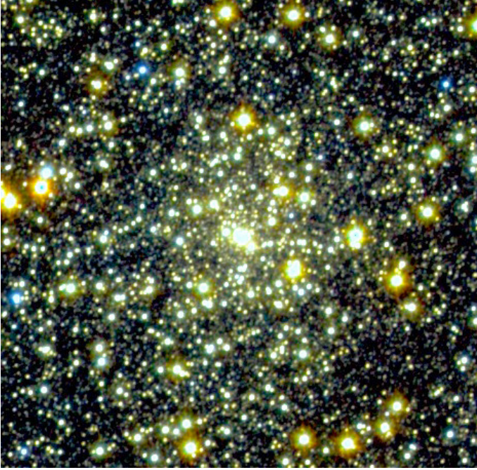
Fig. 1. HP 1 JHK_s -combined colour image from the VVV survey. The image has size of 2 \times 2 arcmin 2 . North is at 45° anticlockwise.
