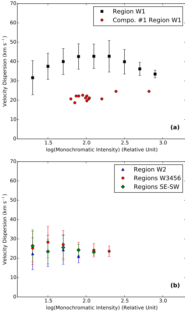
Figure 10. (I - \sigma) diagnostic diagram for the W1 complex (top panel) and for the other complexes in NGC 454 W (bottom panel). The \sigma values are averaged over intensity bins. Red dots on W1 complex show the main component in line profile decomposition shown in Figure 9.
