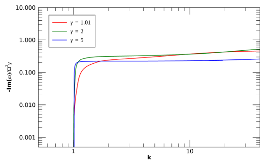
Figure 14. Growth rate of the poloidal buoyancy mode as a function of k for \alpha = 1 , P_c = 1 , and \gamma_c = 1.01, 2, 5 . The growth rate is normalized by \gamma_c \Omega_c^2 . The three different curves refer to three different values of \gamma_c as indicated in the legend. M_a is different for the three curves and for each curve has the value at which the maximum growth rate is found at fixed k : M_a = 1.8, 5.72, 14.2 , respectively, for \gamma_c = 1.01, 2, 5 .
