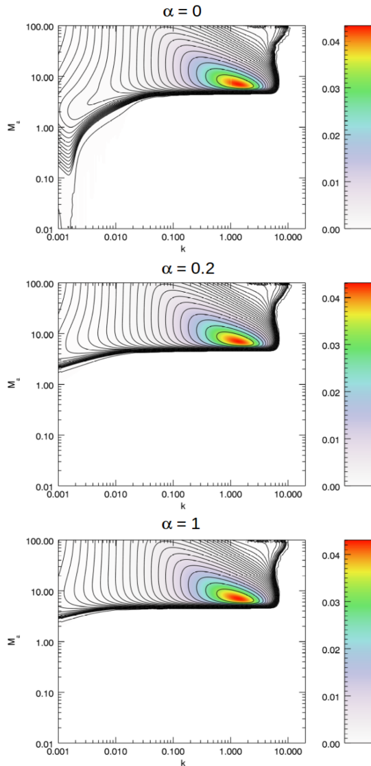
Figure 6. Same as in Fig. 4, but for \gamma_c = 10 and P_c = 10 .
