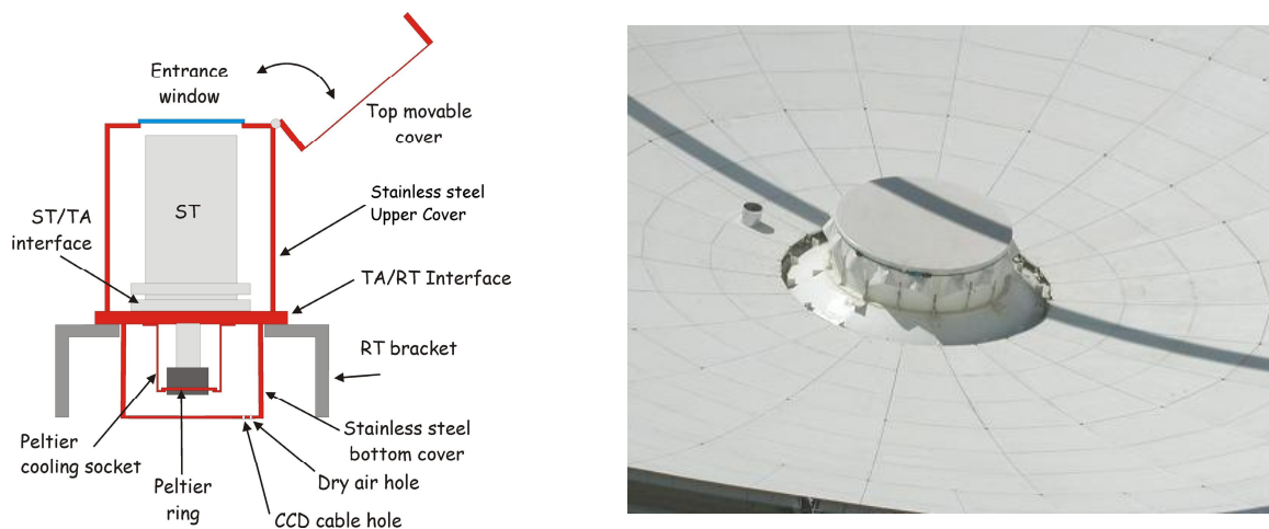
Fig. 3. Left ): Sketch of the Star Tracker (ST). Right ): Photo of the Star Tracker mounted on the 32 m Medicina antenna (on the left of the primary mirror vertex).
