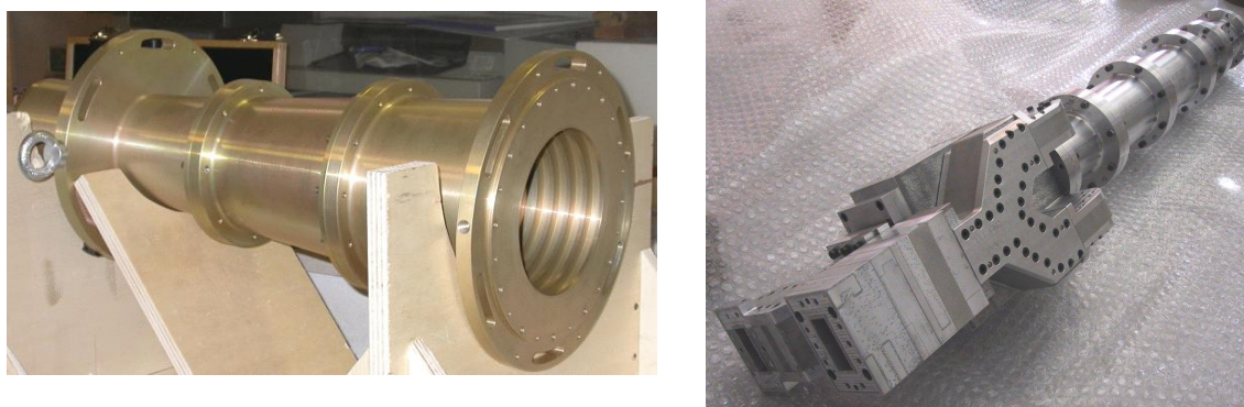
Fig. 6. The horn (left) and the chain of marker injector-polarizer-omt (right) for the 5.7-7.7 GHz receiver.
