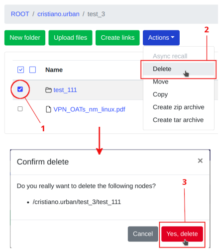
Figure 10: Deleting a container node.
