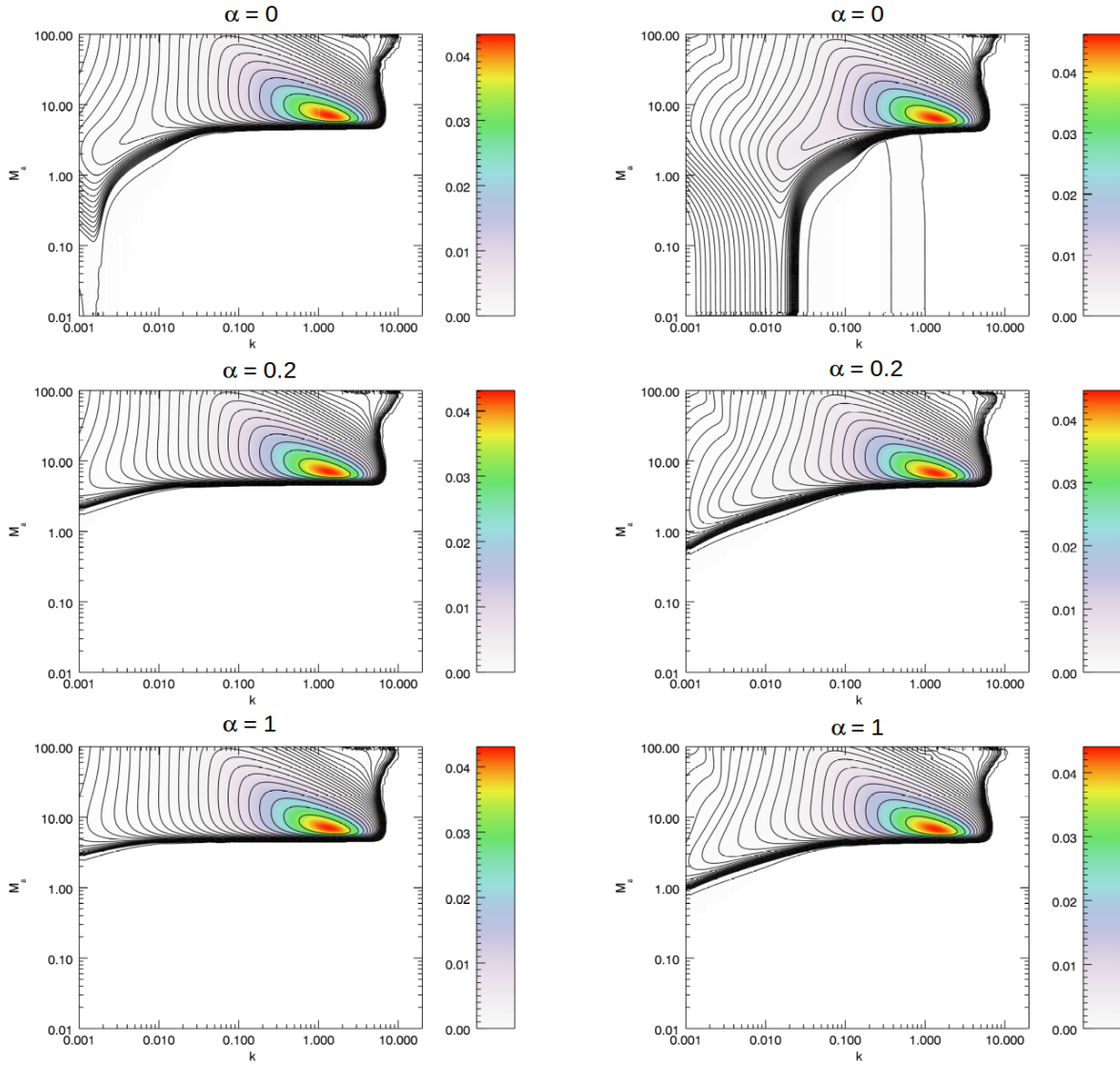
Figure 7. Same as in Fig. 4, but for \gamma_c = 10 and P_c = 1 .
