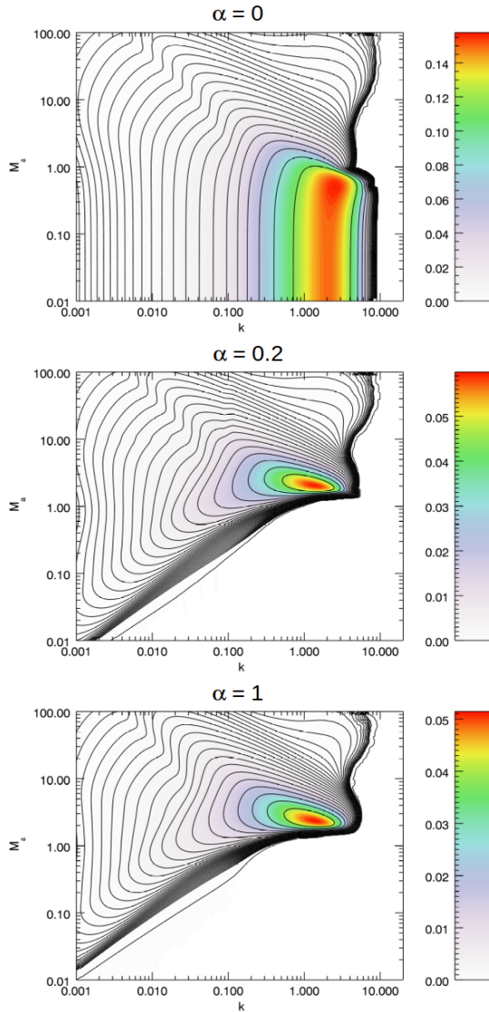
Figure 8. Same as in Fig. 4, but for \gamma_c = 10 and P_c = 0.01 .
