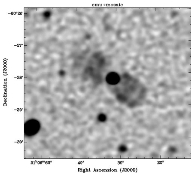
Figure 13. EMU-PS image of the edge-brightened double-lobe radio galaxy EMU PD J210931.3-602806. No redshift is available for this source.
