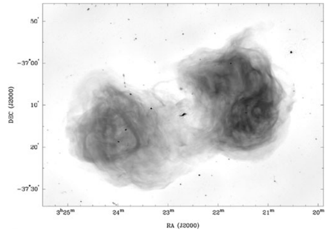
Figure 12. ASKAP 944 MHz radio continuum image of the double-lobe radio galaxy Fornax A, from unpublished ASKAP data.
