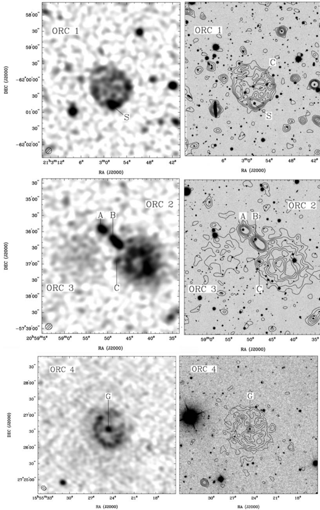
Figure 1. ASKAP radio continuum images at 944 MHz of ORCs 1–3 from the EMU Pilot Survey (Norris et al. 2020) and at 325 MHz of ORC 4 from GMRT archival data. On the left are greyscale images, with the synthesized beam shown in the bottom left corner, and radio contours overlaid onto DES optical images on the right, as described in the text. The contour levels for ORC 1 and ORC 2 are 45, 90, 135, 180, 225, and 270 \mu\text{Jy beam}^{-1} , and contour levels for ORC 4 are 150, 250, 400, 600, and 800 \mu\text{Jy beam}^{-1} . Sources of interest are labelled (see Tables 3 and 4).
