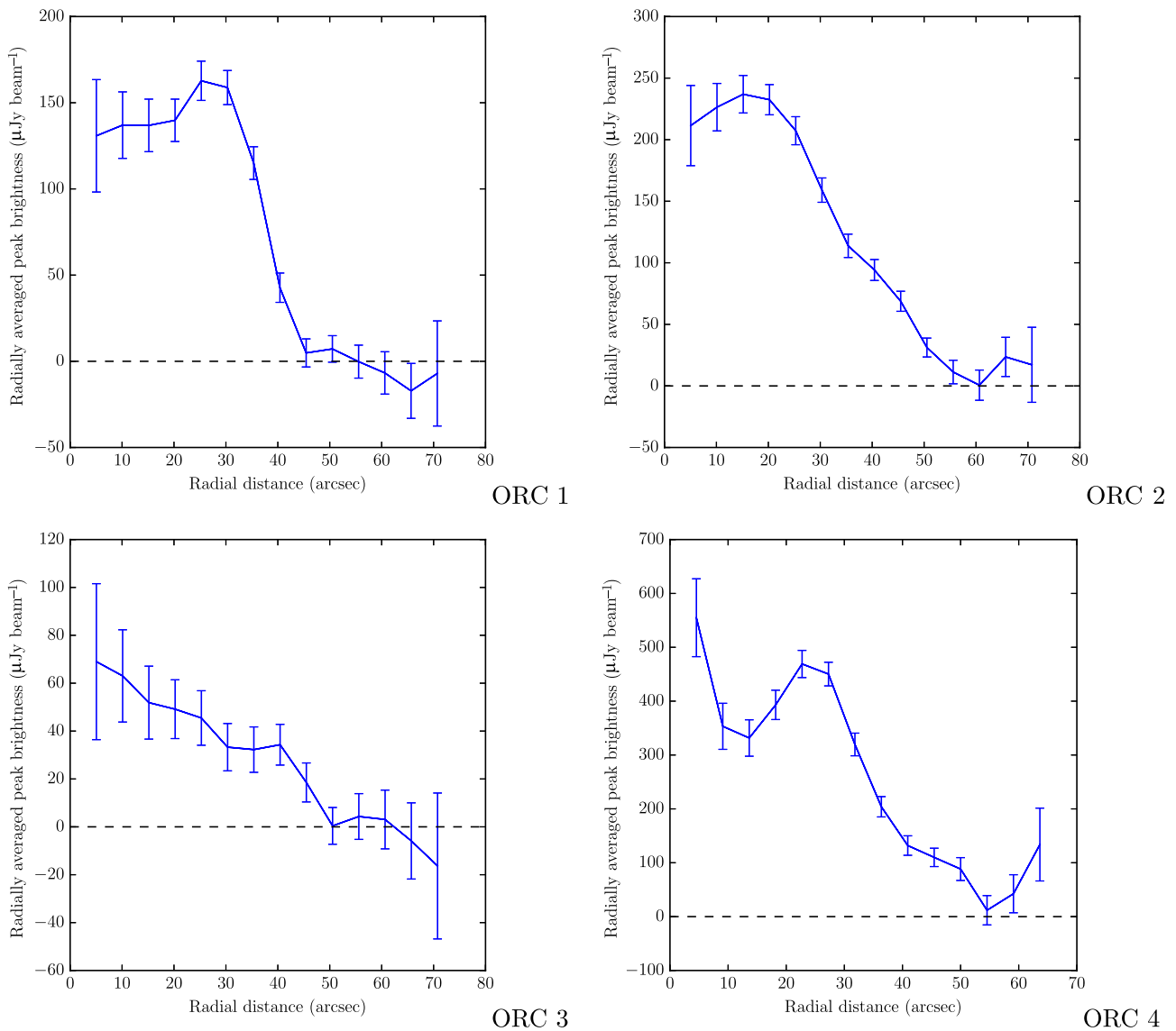
Figure 8. Radial profiles of the diffuse emission of the ORCs, measured from the ASKAP and GMRT data and integrated radially around the ORC, assuming circular symmetry, after removing compact sources A and B in ORC 2. Error bars are \sigma/\sqrt{\text{number of independent beam volumes}} , where \sigma = 25 \mu\text{Jy beam}^{-1} for the EMU data (ORCs 1, 2, and 3), and 60 \mu\text{Jy beam}^{-1} for the uGMRT data (ORC 4).
