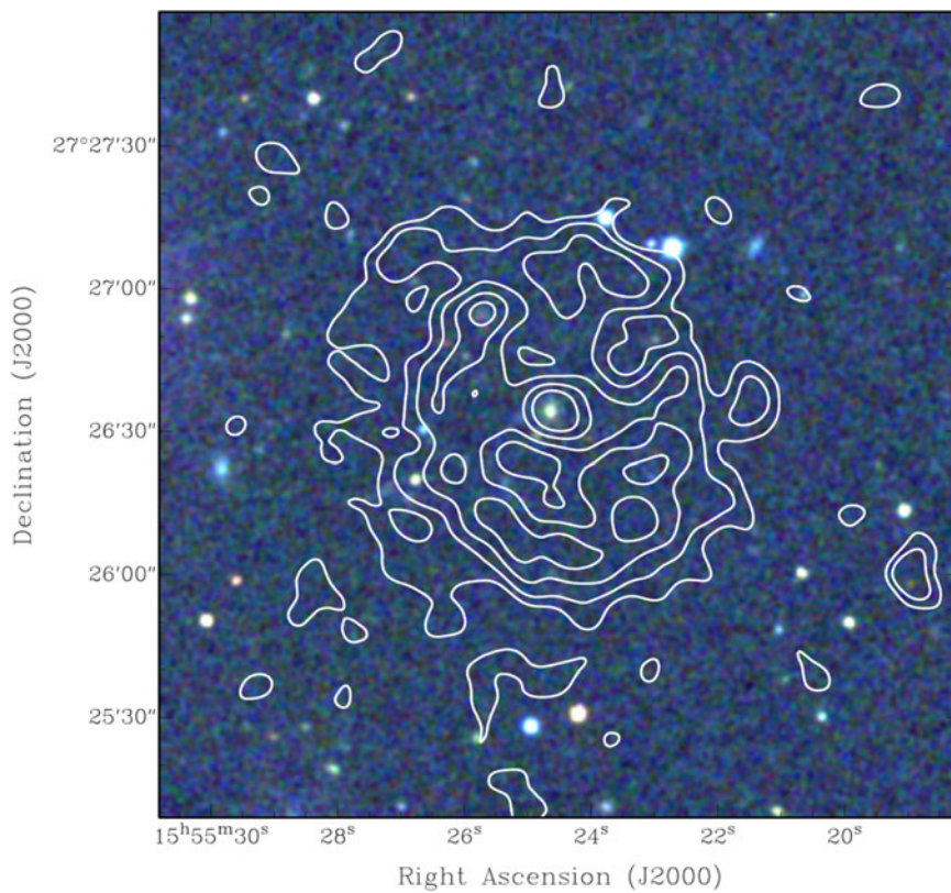
Figure 7. GMRT radio continuum image of ORC 4 (contours; see Figure 1) overlaid onto a SDSS 3-color composite image; SDSS gri -bands are colored blue, green, and red, respectively.
