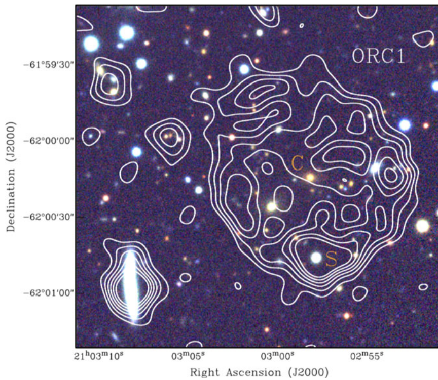
Figure 5. ASKAP radio continuum image of ORC 1 (contours; see Figure 1) overlaid onto a DES 3-color composite image; DES gri -bands are colored blue, green, and red, respectively. We identify two galaxies of interest: ‘C’ lies near the centre of ORC 1 and ‘S’ coincides with the southern radio peak (see Table 3).
