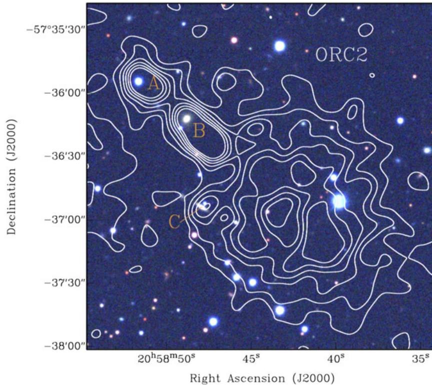
Figure 6. ASKAP radio continuum image of ORC 2 (contours; see Figure 1) overlaid onto a DES 3-color composite image; DES gri -bands are colored blue, green, and red, respectively. We identify three sources of interest, annotated A, B, and C (see Table 4).
