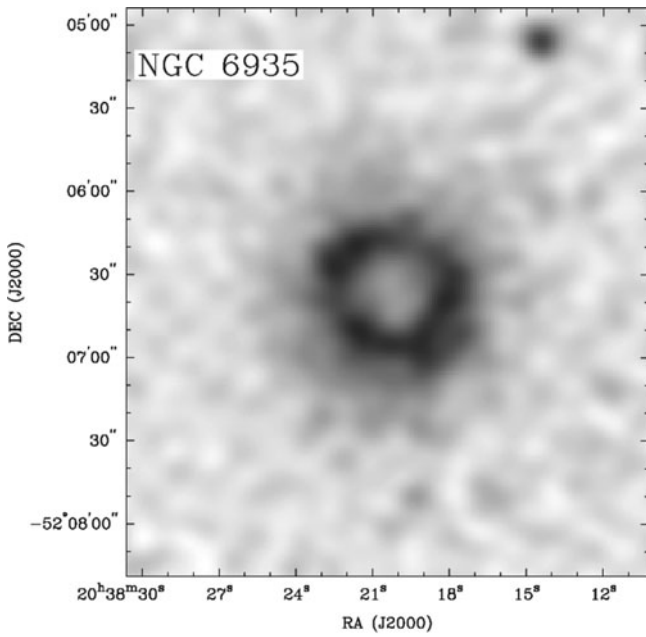
Figure 10. ASKAP 944 MHz radio continuum image of the face-on, star-forming galaxy NGC 6935 ( v = 4\,543\text{ km s}^{-1} ), as observed in the EMU-PS. The ring is about 2 kpc in diameter.
