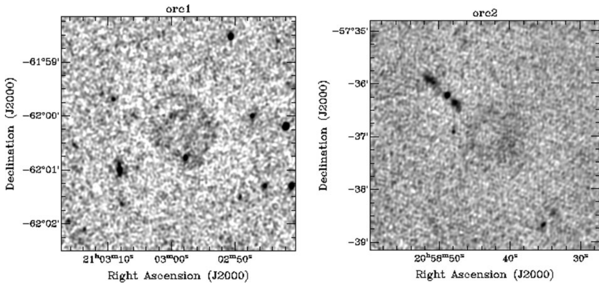
Figure 4. ATCA radio continuum images of ORCs 1–3 at a frequency of 2.1 GHz. The image rms is about 12 \mu\text{Jy beam}^{-1} in both images. ORCs 1 and 2 are only faintly visible in these higher frequency images because of their steep spectral index and higher resolution, while ORC 3 is below the rms noise level. This image shows that sources A and B in ORC 2 are the two halves of an FRI radio galaxy.
