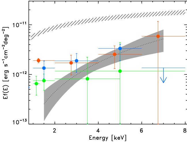
Fig. 10. Spectrum of the unresolved CXRB: comparison with previous measures. The gray area is the result of the present work. Green points are from Hickox & Markevitch (2007) ; blue points are from Luo et al. (2011) , with the blue arrow indicating the 1\sigma upper limit; red points from Worsley et al. (2006) . The dashed area represents the total CXRB emission as measured by Swift ( Moretti et al. 2009 ).
