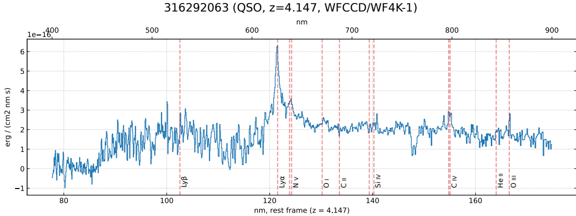
Figure 5. Spectrum, resampled at 250 km/s, of the brightest z\sim 4 QSO in the sample, with some AGN emission lines
