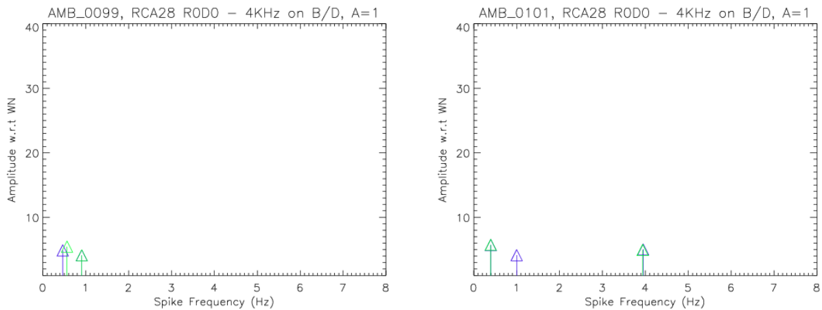
Figure 31 SFT in Cannes (left) vs WFT in Milan (right), RCA28 in which 4KHz is on B/D and A/C = 1.
