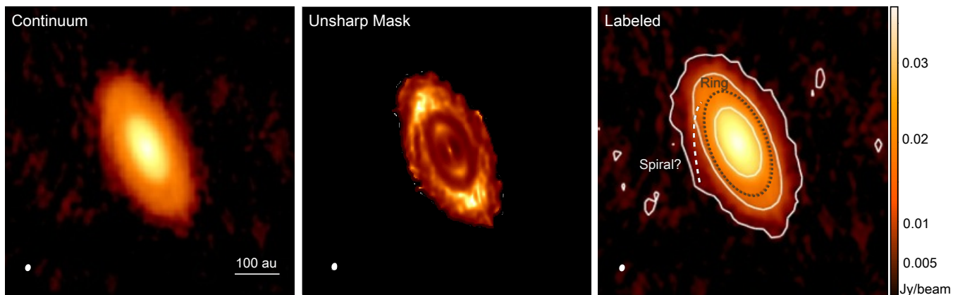
Fig. 1. Continuum emission toward DG Tau B at 235 GHz (1.27 mm). Left panel: Original image in logarithmic color stretch. Middle panel: Same image after applying unsharp masking, i.e., the subtraction from the original image of the same image smoothed by 0.1'' . Right panel: Labeled version of the same image. The isophote curves at 3\sigma , 25\sigma , and 100\sigma (with \sigma = 0.034 mJy beam -1 ) are shown together with the location of the broad ring (brown) and a putative spiral arm (gray) inferred from the unsharp masked image.
