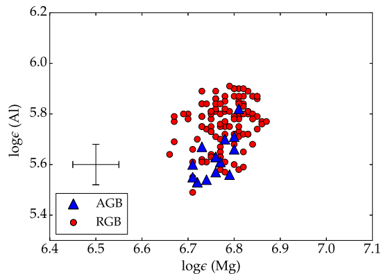
Figure 6. Same as Fig. 5, but for Mg and Al abundances.
