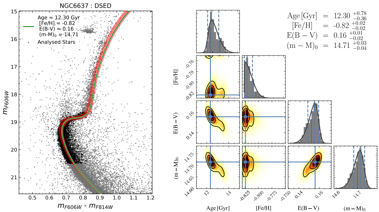
Figure 8. Same as Figure 7 for DSED isochrones.
