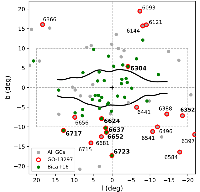
Figure 1. Location in Galactic coordinates of the GCs presented in Harris (1996, 2010 edition) catalog, within |\ell| < 22^\circ and |b| < 22^\circ . The open red circles correspond to the 56 GCs observed in the GO-13297 program. The black contours correspond to the COBE/DIRBE outline of the peanut bulge (Weiland et al. 1994; Jönsson et al. 2017), and the dashed lines delimit the central region with |\ell| < 20^\circ and |b| < 10^\circ . The only six clusters with R_{GC} < 3 kpc and [\text{Fe}/\text{H}] > -1.5 , classified as bulge GCs in Bica et al. (2016, green circles), were selected for this present analysis. NGC 6352, which is classified as an outer bulge GC, was also selected.
