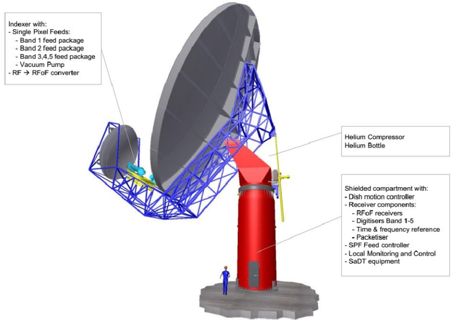
Figure 1: SKA DISH overview
