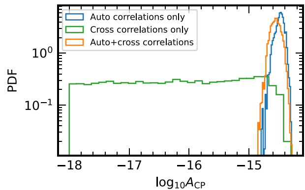
Figure 4. The constraints from the split ORF analysis on the common process amplitude with spectral index fixed to \gamma = 13/3 . The posterior from the autocorrelations is well constrained, while the posterior from the cross-correlations is unconstrained, but prefers amplitudes slightly smaller than the auto-only analysis. The effect of this is seen in the amplitude posterior from the full auto + cross-correlation model, where the posterior peaks at lower amplitude than the auto-only analysis.
