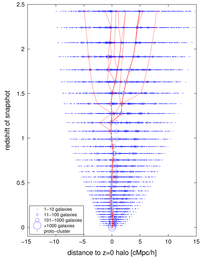
Figure 2. The assembly history of a z \sim 2.5 protocluster. We follow all halos that will eventually become part of the same z = 0 DM halo, i.e., form a cluster. The size of the circles corresponds to the number of galaxies that inhabit a given halo. While at z \sim 2.5 galaxies are mostly centrals themselves, they continuously accrete onto other halos to eventually become satellites in the z = 0 cluster. The protocluster member halos we identify at z \sim 2.5 are highlighted in red.
