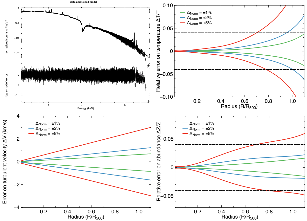
Figure 2. ( Top left ) Example of a spectrum fitted with a biased estimation of the NXB normalisation by \Delta_{Norm}=2\% for an unrealistic 100 Ms observation (to observe systematic effects). Residuals show an underestimation at high energy related to an over-subtraction of the background. Corresponding systematic errors made over the radial profile of the cluster (in units of R_{500} ) for different values of \Delta_{Norm} = \pm 1 (green), 2 (blue) and 5% (red) for temperature ( Top right - relative error), abundances ( Bottom right - relative error) and turbulent velocity ( Bottom left - in km/s). Dashed lines indicate the current 4% requirement accuracy for temperature and abundances.
