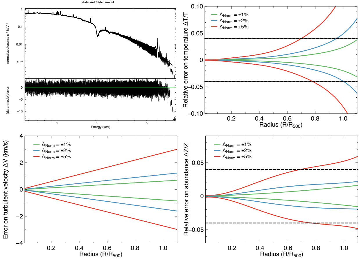
Figure 2. ( Top left ) Example of a spectrum fitted with a biased estimation of the NXB normalisation by \Delta_{Norm}=2\% for an unrealistic 100 Ms observation (to observe systematic effects). Residuals show an underestimation at high energy related to an over-subtraction of the background. Corresponding systematic errors made over the radial profile of the cluster (in units of R_{500} ) for different values of \Delta_{Norm} = \pm 1 (green), 2 (blue) and 5% (red) for temperature ( Top right - relative error), abundances ( Bottom right - relative error) and turbulent velocity ( Bottom left - in km/s). Dashed lines indicate the current 4% requirement accuracy for temperature and abundances.
