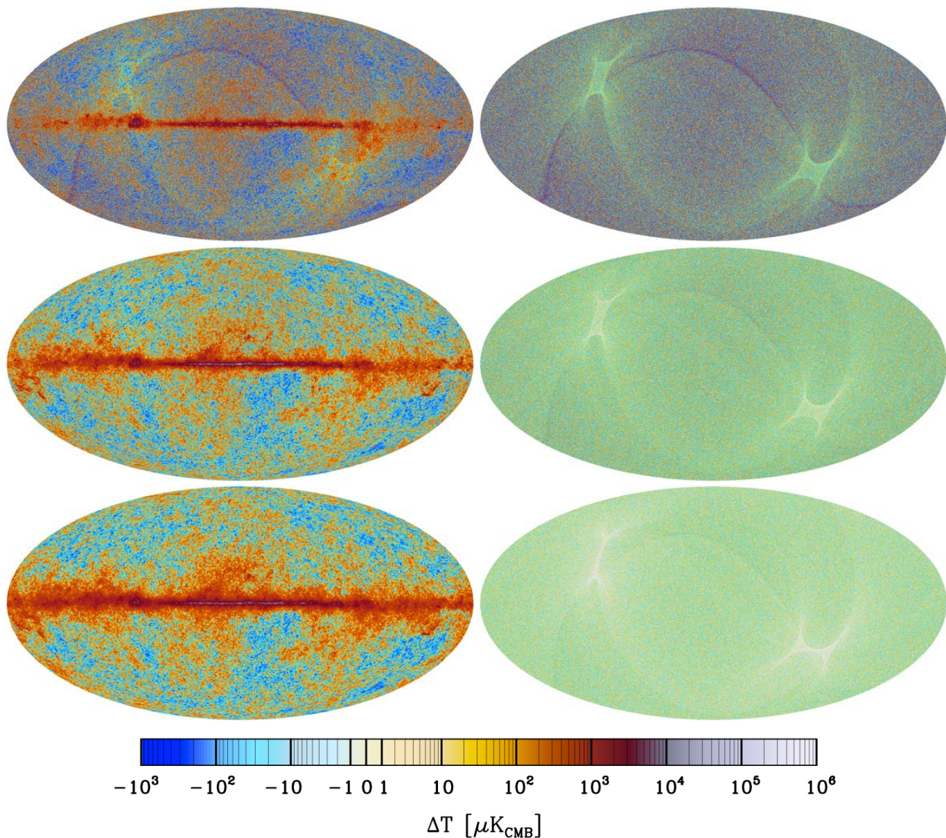
Fig. 2. Sky maps used in the analysis of Planck data consistency. Top row: 70 GHz. Middle row: 100 GHz. Bottom row: 143 GHz. Left column: signal maps. Right column: noise maps derived from half-ring differences. All maps are N_{\text{side}} = 2048 . These are the publicly-released maps corrected for monopole and dipole terms as described in the text. The impression of overall colour differences between the maps is due to the interaction between noise, the colour scale, and display resolution. For example, the larger positive and negative swings between pixels in the 70 GHz noise map pick up darker reds and blues farther from zero. Smaller swings around zero in the 100 and 143 GHz noise maps result in pastel yellows and blues in adjacent pixels, which when displayed at less than full-pixel resolution give an overall impression of green, a colour not used in the colour bar.
