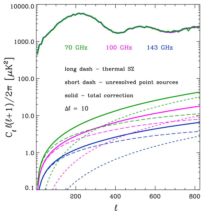
Fig. 8. Estimates of the residual thermal SZ and unresolved radio and infrared source residuals that must be removed.
