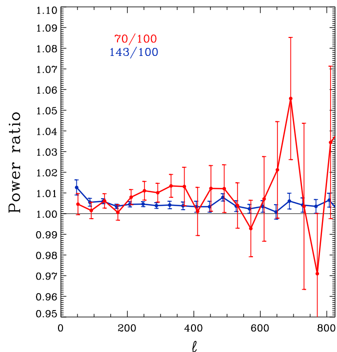
Fig. 9. Same as the bottom middle panel of Fig. 6, but corrected for differences in unresolved-source residuals (see text). We have not tried to account for uncertainties in the foreground correction itself; however, since the correction is small, the effect on the uncertainties would be small.
