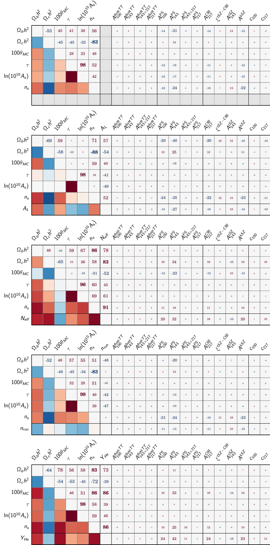
Figure 45. Parameter correlations for PlikTT+lowTEB, including some \Lambda CDM extensions. The leftmost column is identical to Fig. 44 and is repeated here to ease comparison. Including extensions to the \Lambda CDM model changes the correlations between the cosmological parameters, sometimes dramatically, as can be seen in the case of A_L . There is no correlation between the cosmological parameters (including the extensions) and the dust amplitude parameters. In most cases, the extensions are correlated with the remaining foreground parameters (and in particular with the point-source amplitudes at 100 and 143 GHz, and with the level of CIB fluctuations) with a strength similar to those of the other cosmological parameters (i.e., less than 30 %). Y_{\text{He}} exhibits a stronger sensitivity to the point-source levels.
