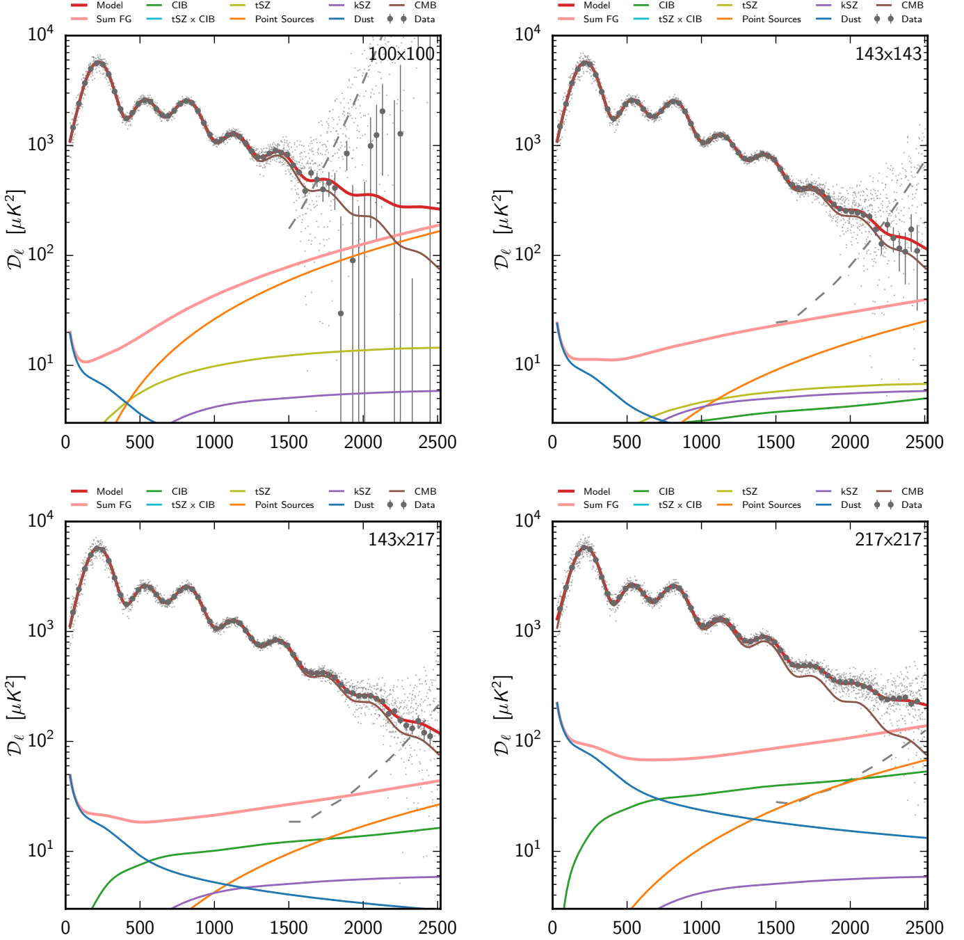
Figure 18. Best model (CMB and foreground) in each of the cross-spectra used for the temperature high- \ell likelihood. The small light grey points show the unbinned data point, and the dashed grey line show the square root of the noise contribution to the diagonal of the unbinned covariance matrix.
