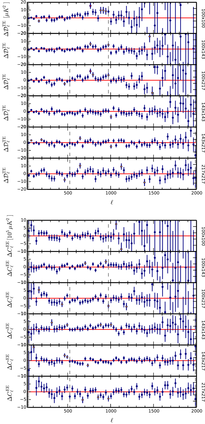
Figure 40. Residual frequency power spectra after subtraction of the PlikTT+tauprior best-fit model. We clean Galactic dust from the spectra from using the best-fit solution of PlikTT,TE,EE+tauprior. The residuals are relative to the baseline HM power spectra (blue points, except for those that deviate by at least 2\sigma or 3\sigma , which are shown in orange or red, respectively). The vertical dashed lines delimit the \ell ranges retained in the likelihood. Upper: TE power spectra. Lower: EE power spectra.
