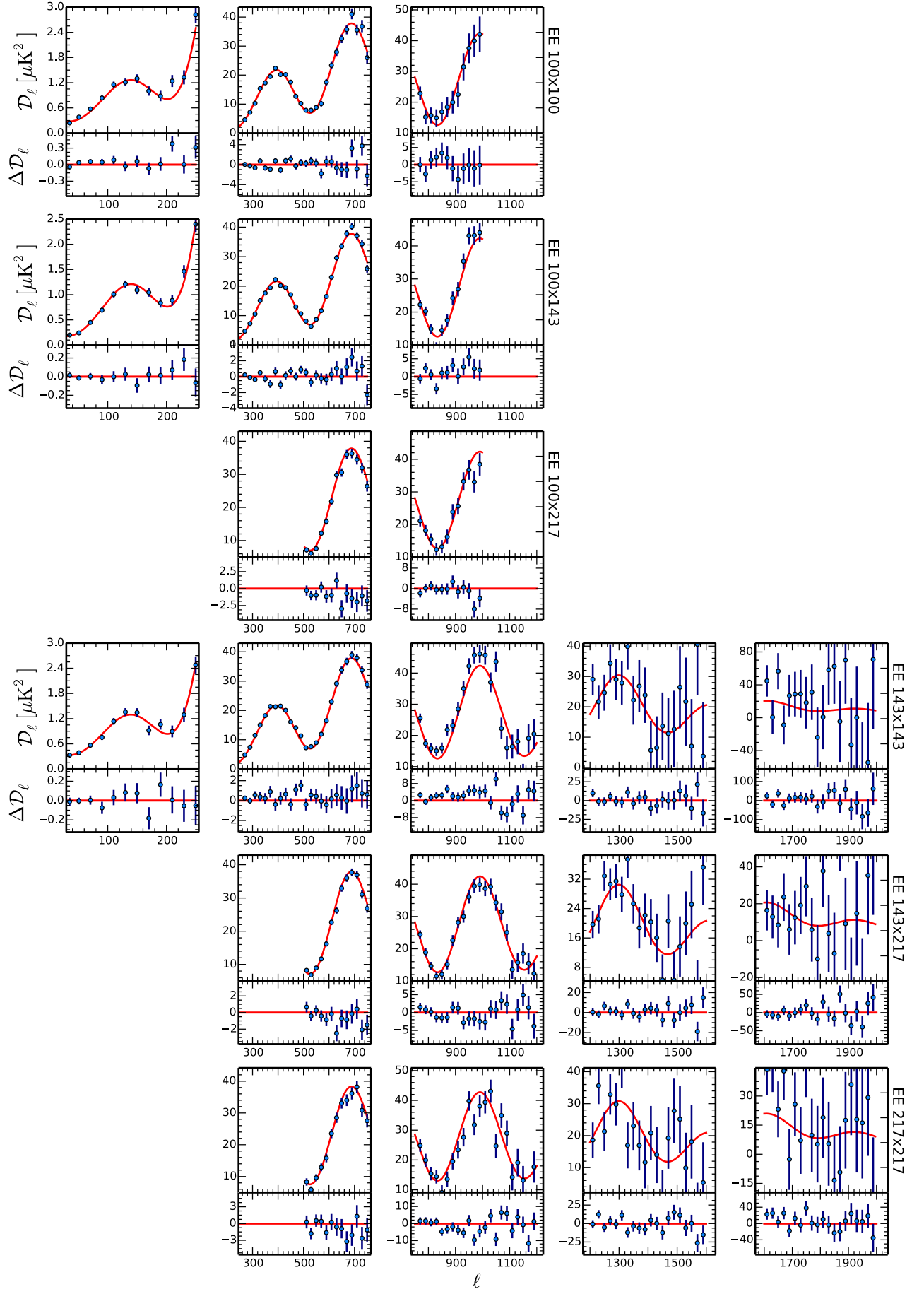
Figure C.6. Same as Fig. C.5, but for EE.
