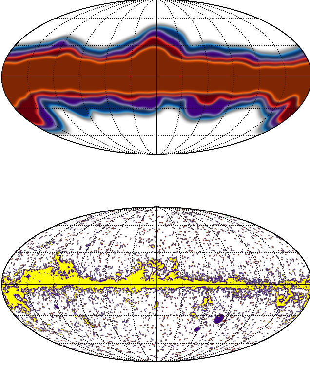
Figure 12. Top: Apodized Galactic masks: G41 (blue), G50 (purple), G60 (red), and G70 (orange); these are identical to the polarization masks P41 (used at 217 GHz), P50 (143 GHz), P70 (100 GHz). Bottom: Extragalactic-object masks for 217 GHz (purple), 143 GHz (red), and 100 GHz (orange); the CO mask is shown in yellow.
