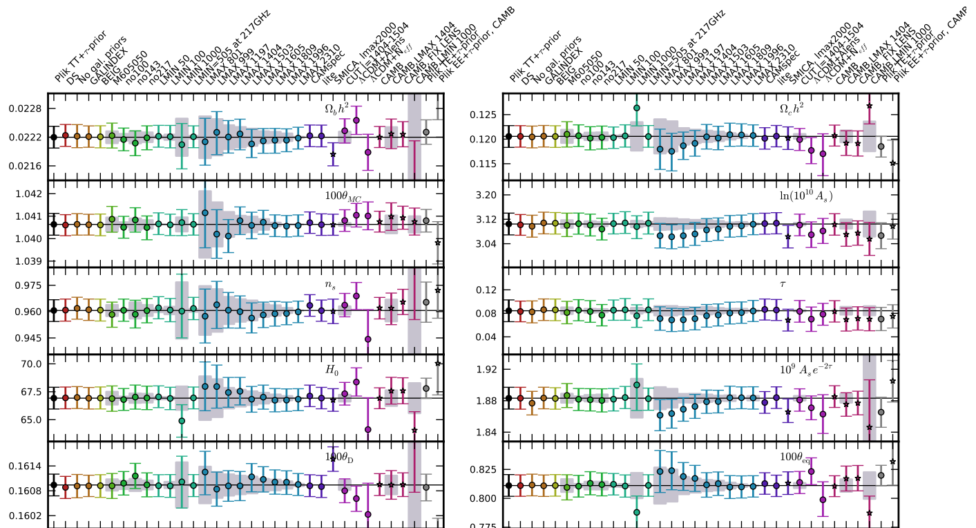
Figure 35. Marginal mean and 68 % CL error bars on cosmological parameters estimated with different data choices for the Plik likelihood, in comparison with results from alternate approaches or model. We assume a \Lambda CDM model and use variations of the PlikTT likelihood in most of the cases, in combination with a prior \tau = 0.07 \pm 0.02 (using neither low- \ell temperature nor polarization data). The “PlikTT+tauprior” case (black dot and thin horizontal black line) indicates the baseline (HM, \ell_{\min} = 30 , \ell_{\max} = 2508 ), while the other cases are described in Sect. 4.1 (and 4.2, 5.6, E.4). The grey bands show the standard deviation of the expected parameter shift, for those cases where the data used is a sub-sample of the baseline likelihood (see Eq. 53). All the results were run with PICO except for few ones that were run with CAMB, as indicated in the labels.
