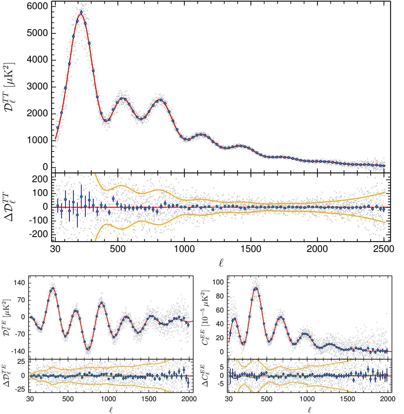
Figure 28. Plik 2015 co-added TT , TE , and EE spectra. The blue points are for bins of \Delta\ell = 30 , while the grey points are unbinned. The lower panels show the residuals with respect to the best fit PlikTT+tauprior \Lambda CDM model. The yellow lines show the 68 % unbinned error bars. For TE and EE , we also show the best-fit beam-leakage correction (green line; see text and Fig. 23).
