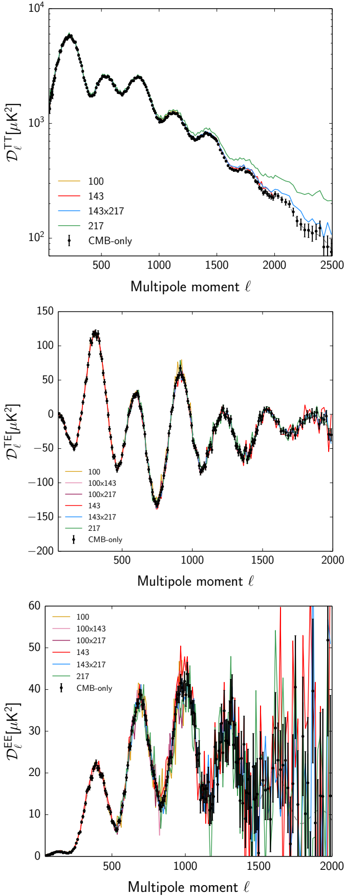
Figure C.12. Planck multi-frequency power spectra (solid coloured lines) and extracted CMB-only spectra (black points).
