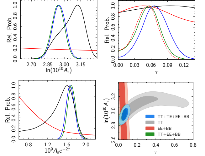
Figure 6. Likelihoods for parameters from low- \ell data. Panels 1–3: One-dimensional posteriors for \log[10^{10} A_s] , \tau , and A_s e^{-2\tau} for the several sub-blocks of the likelihood, for cases 1 (blue), 2 (black), 3 (red), and 4 (green) — see text for definitions; dashed red is the same as case 3 but imposes a sharp prior 10^9 A_s e^{-2\tau} = 1.88 . Panel 4: Two-dimensional posterior for \log[10^{10} A_s] and \tau for the same data combinations; shading indicates the 68 % and 95 % confidence regions.
