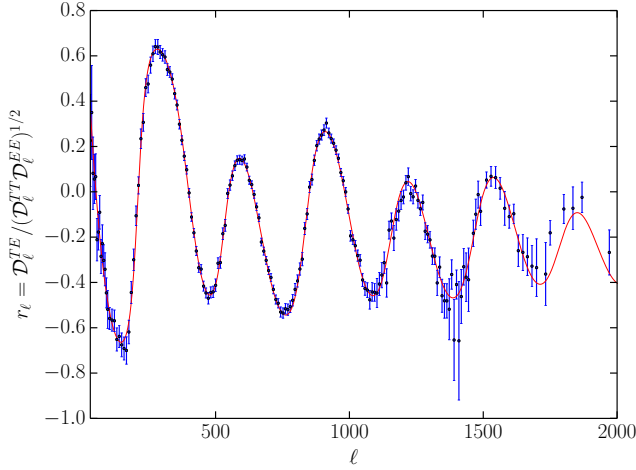
Figure E.2. Pearson correlation coefficient for T and E . The red curve is the theoretical best-fit to the Planck TT, TE, EE+lowP data. The blue points are the binned Planck data described in this paper. Data points with negative values for EE , or low S/N in polarization (specifically S/N < 1 ) are omitted, which leads to an apparent bias between the theory curve and the data at the highest multipoles. The error bars here are calculated assuming a Gaussian distribution for the TT , TE , and EE power values, which should be a reasonable approximation at high \ell . The Pearson coefficient is also normally distributed at high \ell .
