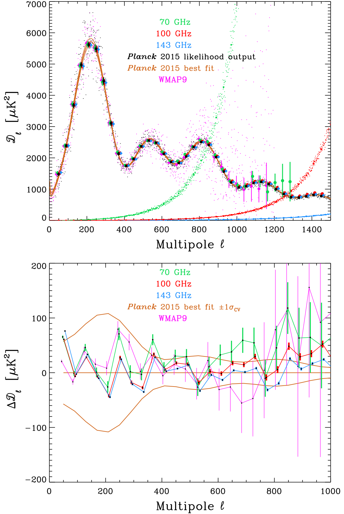
Figure 48. Comparison of Planck and WMAP-9 CMB power spectra. Top: Direct comparison. Noise spectra are derived from the half-ring difference maps. Bottom: Residuals with respect to the Planck \Lambda CDM best-fit model. The error bars do not include the cosmic variance contribution (but the (brown) 1\text{-}\sigma contour lines for the Likelihood best fit model do).
