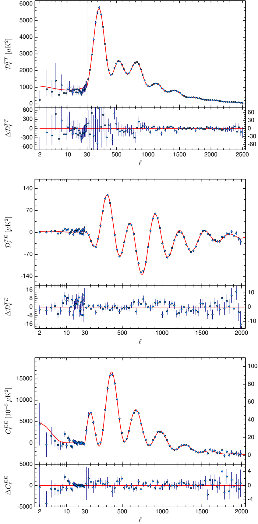
Figure 50. Planck 2015 CMB spectra, compared with the base \Lambda CDM fit to PlanckTT+lowP data (red line). The upper panels show the spectra and the lower panels the residuals. In all the panels, the horizontal scale changes from logarithmic to linear at the “hybridization” scale, \ell = 29 (the division between the low- \ell and high- \ell likelihoods). For the residuals, the vertical axis scale changes as well, as shown by different left and right axes. We show \mathcal{D}_\ell = \ell(\ell + 1)C_\ell/(2\pi) for TT and TE , but C_\ell for EE , which also has different vertical scales at low- and high- \ell .
