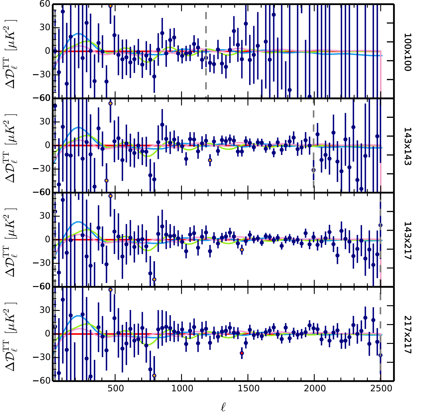
Figure 32. Residuals in the half-mission TT power spectra after subtracting the PlikTT+tauprior \Lambda CDM best-fit model (blue points, except for those which differ by at least 2 or 3\sigma , which are coloured in orange or red, respectively). The light blue line shows the difference between the best-fit model obtained assuming a \Lambda CDM+ A_L model and the \Lambda CDM best-fit baseline; the green line shows the difference of best-fit models using the \ell_{\max} = 999 likelihood (fixing the foregrounds to the baseline solution) minus the baseline best-fit (both in the \Lambda CDM framework); while the pink line is the same as the green one but for \ell_{\max} = 1404 instead of \ell_{\max} = 999 ; see text in Sect. 4.1. For the TE and EE spectra, see Fig. 40.
