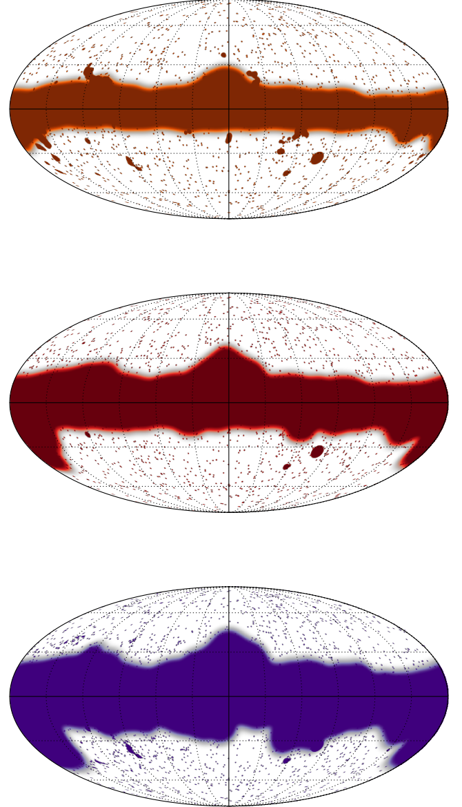
Figure 13. Top to bottom: temperature masks for 100 GHz (T66), 143 GHz (T57) and 217 GHz (T47). The colour scheme is the same as in Fig. 12.
