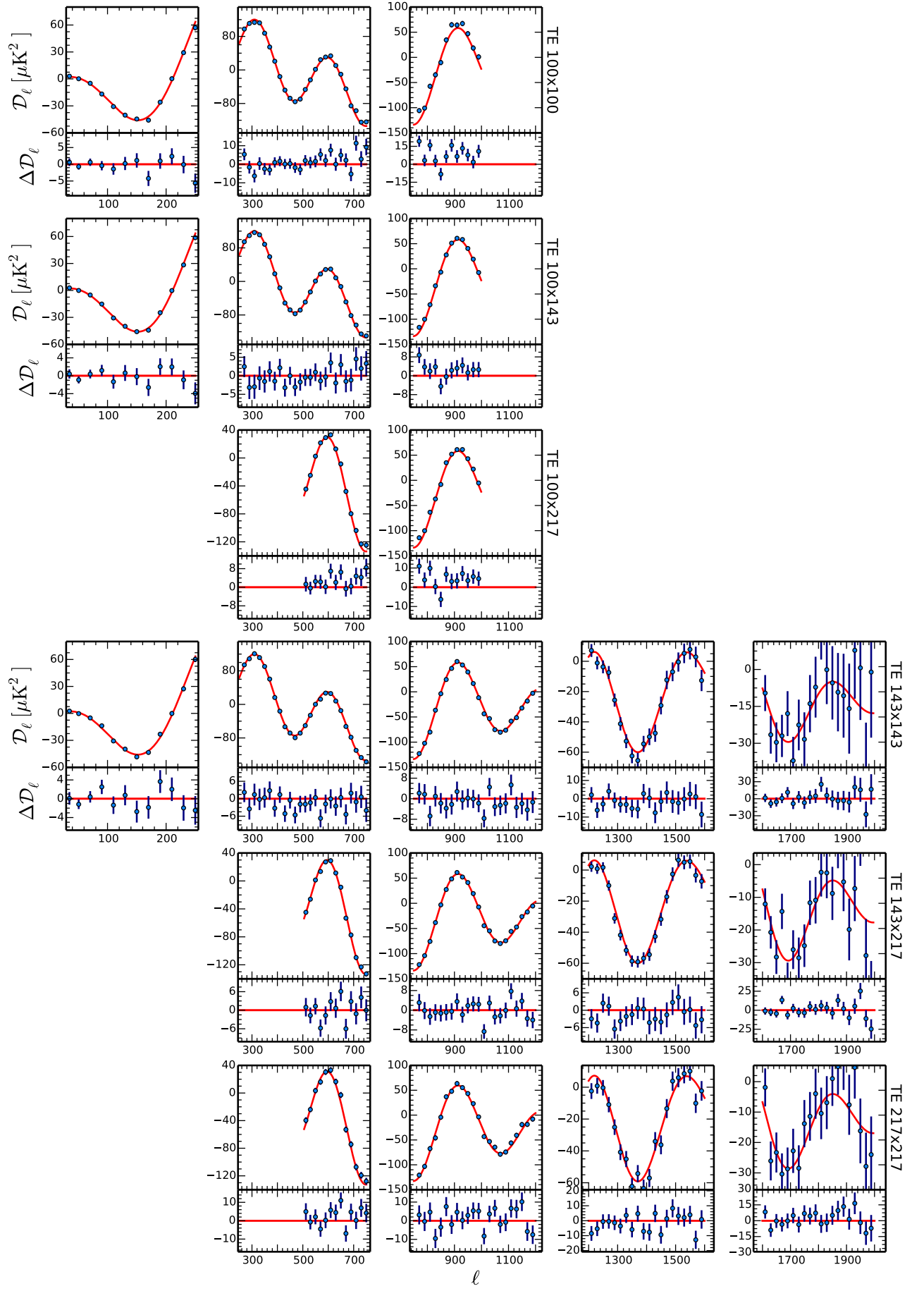
Figure C.7. Same as Fig. C.5, but for TE .
