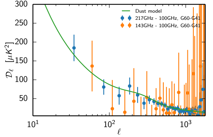
Figure 20. Dust model versus data. In blue, the power spectrum of the double mask difference between 217 GHz and 100 GHz half-mission cross-spectra in masks G60 and G41 (complemented by the joint masks for CO, extended objects, and point sources). In orange, the equivalent spectrum for 143 and 100 GHz. The mask difference enables us to remove the contribution from all the isotropic components (CMB, CIB, and point sources) in the mean. But simple mask differences are still affected by the difference of the CMB in the two masks due to cosmic variance. Removing the 100 GHz mask difference, which is dominated by the CMB, reduces the scatter significantly. The error bars are computed as the scatter in bins of size \Delta\ell = 50 . The dust model (green) based on the 545 GHz data has been rescaled to the expected dust contamination in the 217 GHz mask difference using values from Table 11. The 143 GHz double mask difference is also rescaled to the level of the 217 GHz difference; i.e., it is multiplied by approximately 14. Different multipole bins are used for the 217 GHz and 143 GHz data to improve readability.
