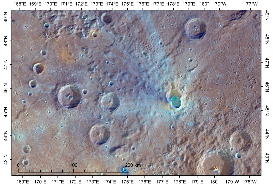
Figure 15. Location 5, with 665 mpp WAC color overlain on 166 mpp NAC mosaic. The rayed crater at 178°E is Ailey.
