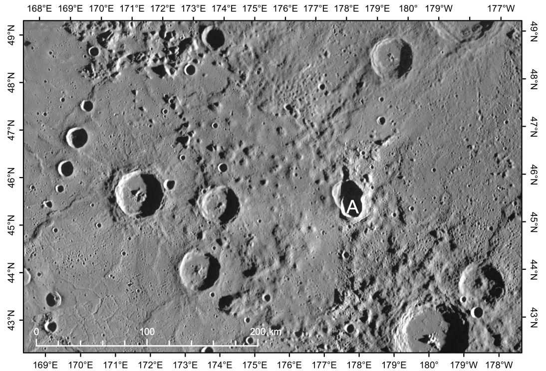
Figure 16. Location 5 166 mpp NAC mosaic. The basin rim runs from the upper left to the lower edge at about 177°E. Note the possible outward facing flow front that can be traced northwestward beyond the rim of Ailey (point A), which is 100 km beyond the Caloris rim.
