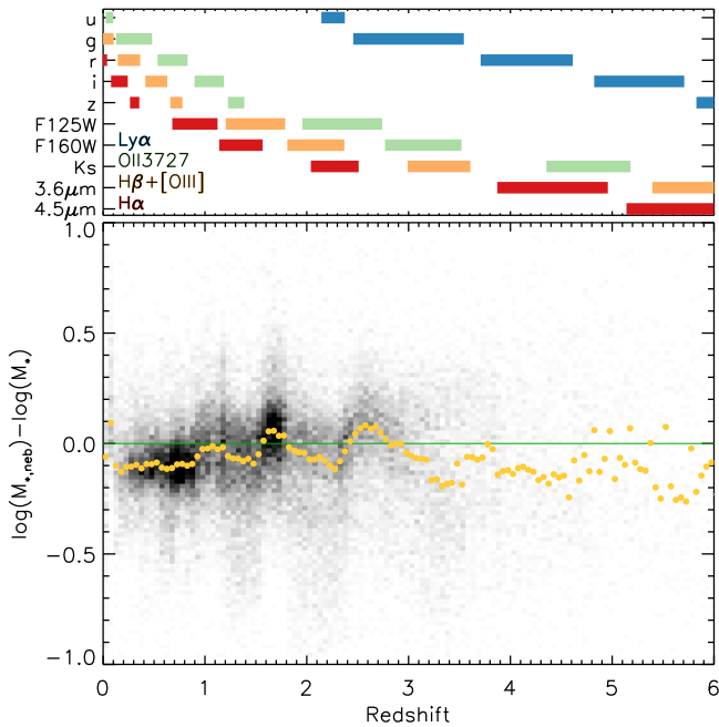
Figure 20. Top panel: cartoon of the presence of four of the stronger emission lines ( \text{Ly}\alpha , \text{O II } \lambda 3727 , \text{H}\beta + [\text{O III}] , and \text{H}\alpha , see the legend) in a subset of bands from the CANDELS multi-wavelength photometric catalog (labeled on the vertical axis), as a function of redshift. Bottom panel: comparison between the stellar mass measurements with and without applying correction for nebular emission contamination. The yellow points mark the median of the difference of the logarithm of stellar mass across redshift, while the horizontal green line marks the 1:1 relation.
