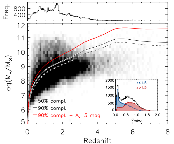
Figure 21. Top panel: photometric redshift distribution of the extended sources ( S_{\text{Extractor CLASS\_STAR}} < 0.7 ) in the catalog in a redshift bin of 0.05. Bottom panel: distribution of the stellar mass as a function of redshifts for the full sample of extended sources ( S_{\text{Extractor CLASS\_STAR}} < 0.7 ) in the CANDELS stellar mass catalog. Overplotted are also the 50% and 90% completeness for a (point source) passively evolving simple stellar population (SSP) from Bruzual & Charlot (2003) together with the 90% completeness of an SSP subject to a dust extinction of A_V = 3 mag, as indicated by the legend. The inset presents the distribution of the spread in \log M_* measurements from the different adopted methods for the full sample (black line) and for objects selected to be at z < 1.5 and z > 1.5 (blue and red filled histograms, respectively, bin width 0.025 dex). The dispersions of the full sample follow a bimodal distribution. The peak with lower stellar mass measurement dispersion is mainly composed of objects at z < 1.5 .
